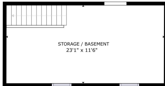
BASEMENT (UNFINISHED) 269 SQ.FT.
