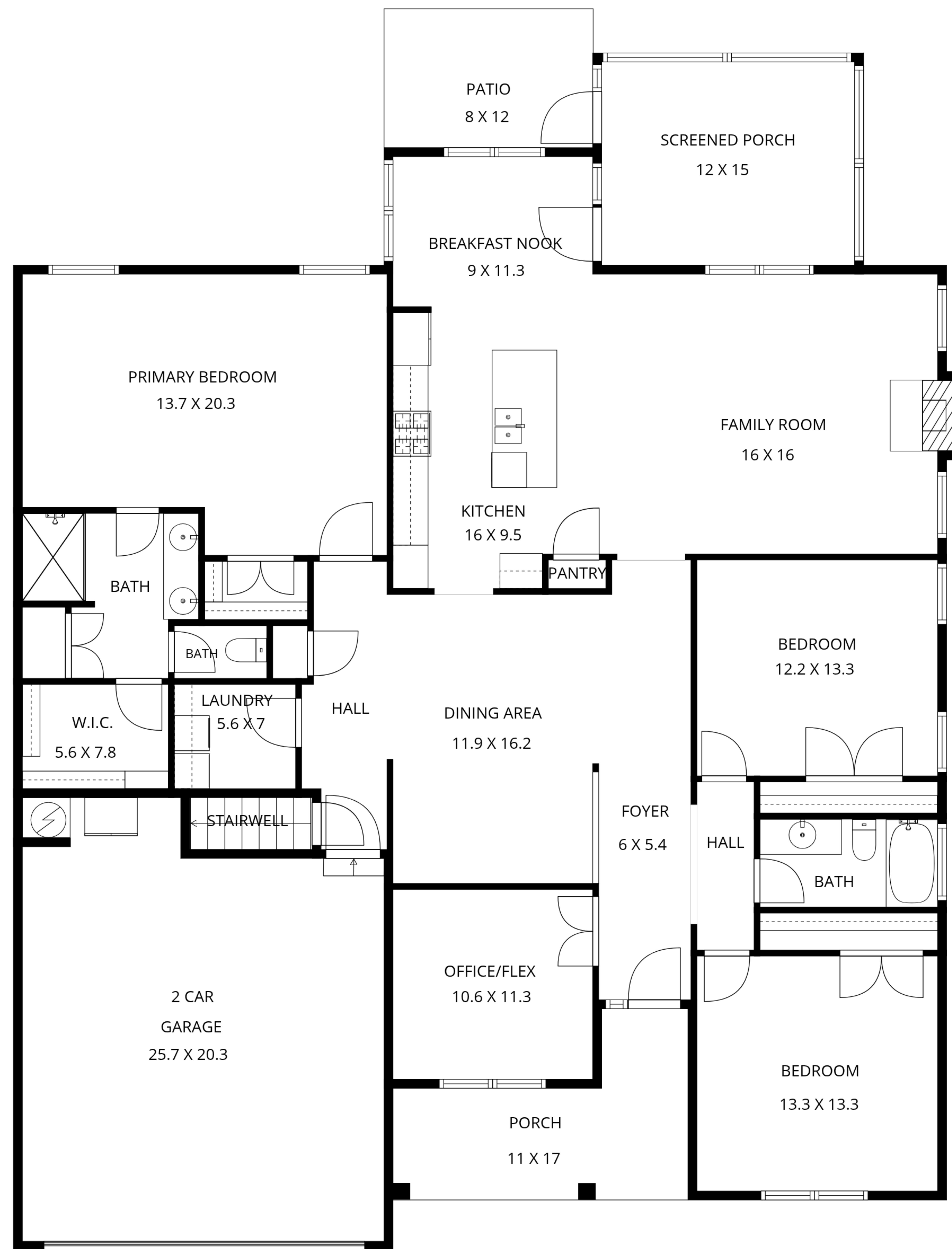
1ST FLOOR
