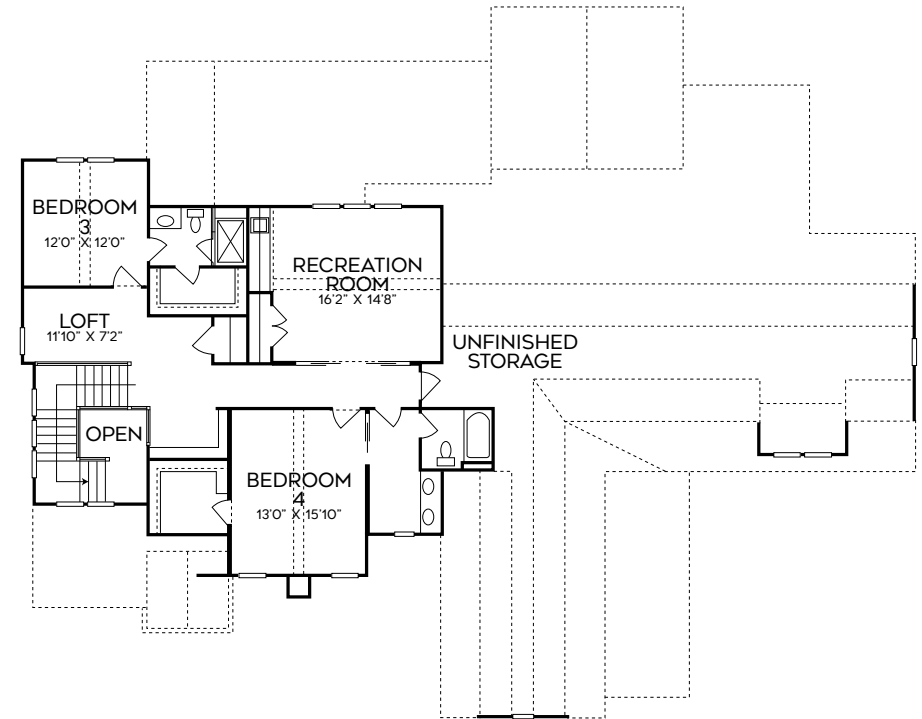
SECOND FLOOR
