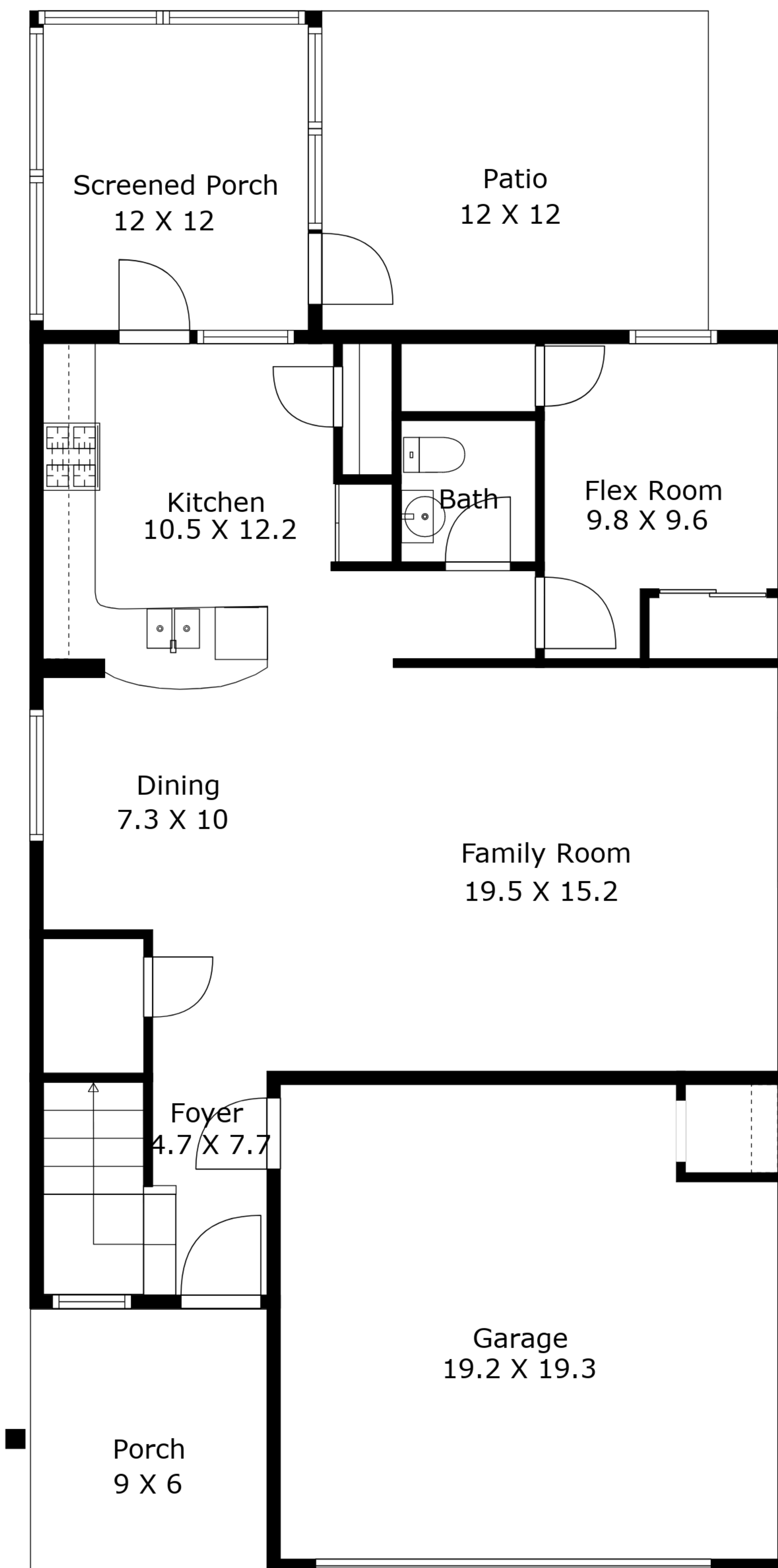
Floor 1
