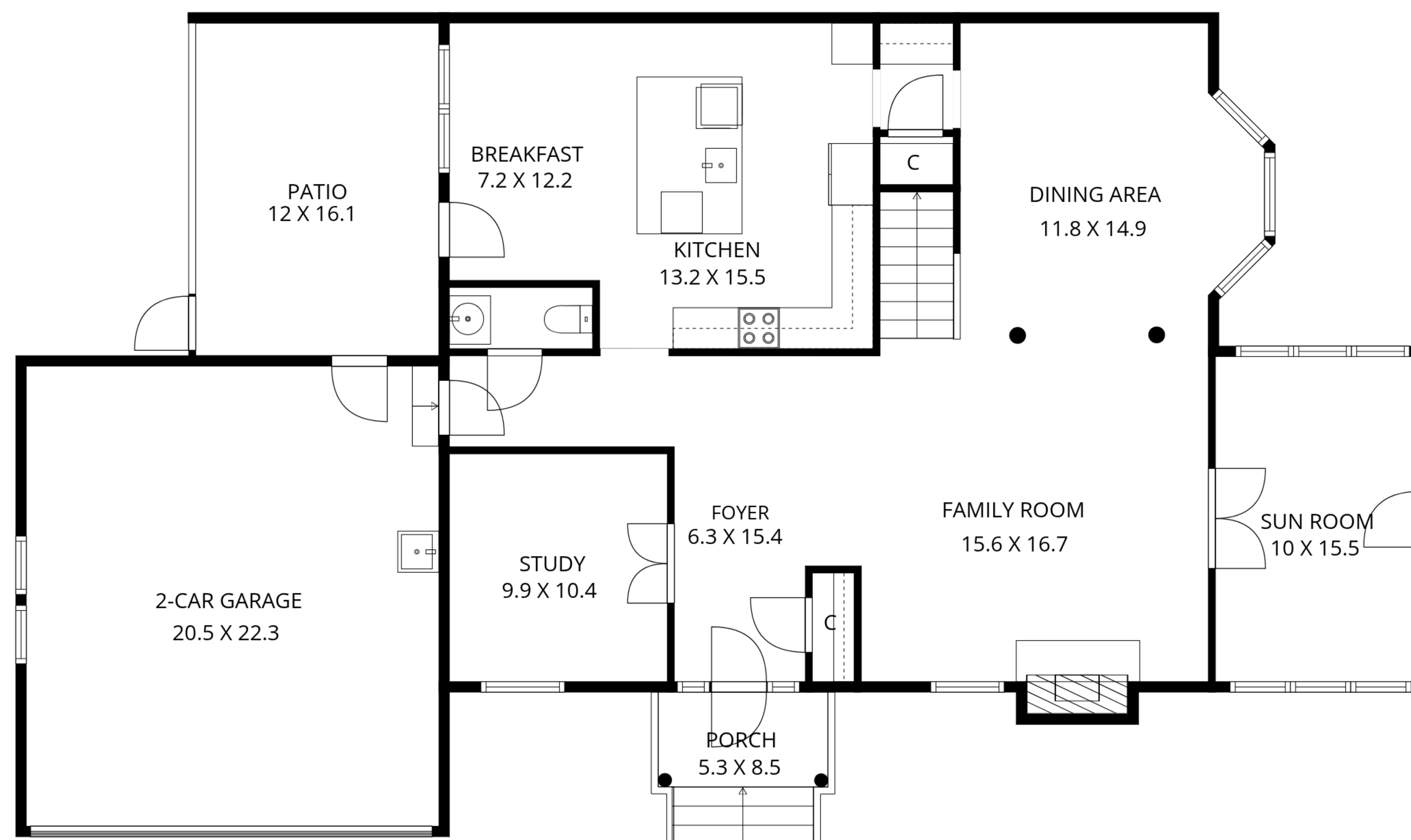
1ST FLOOR
