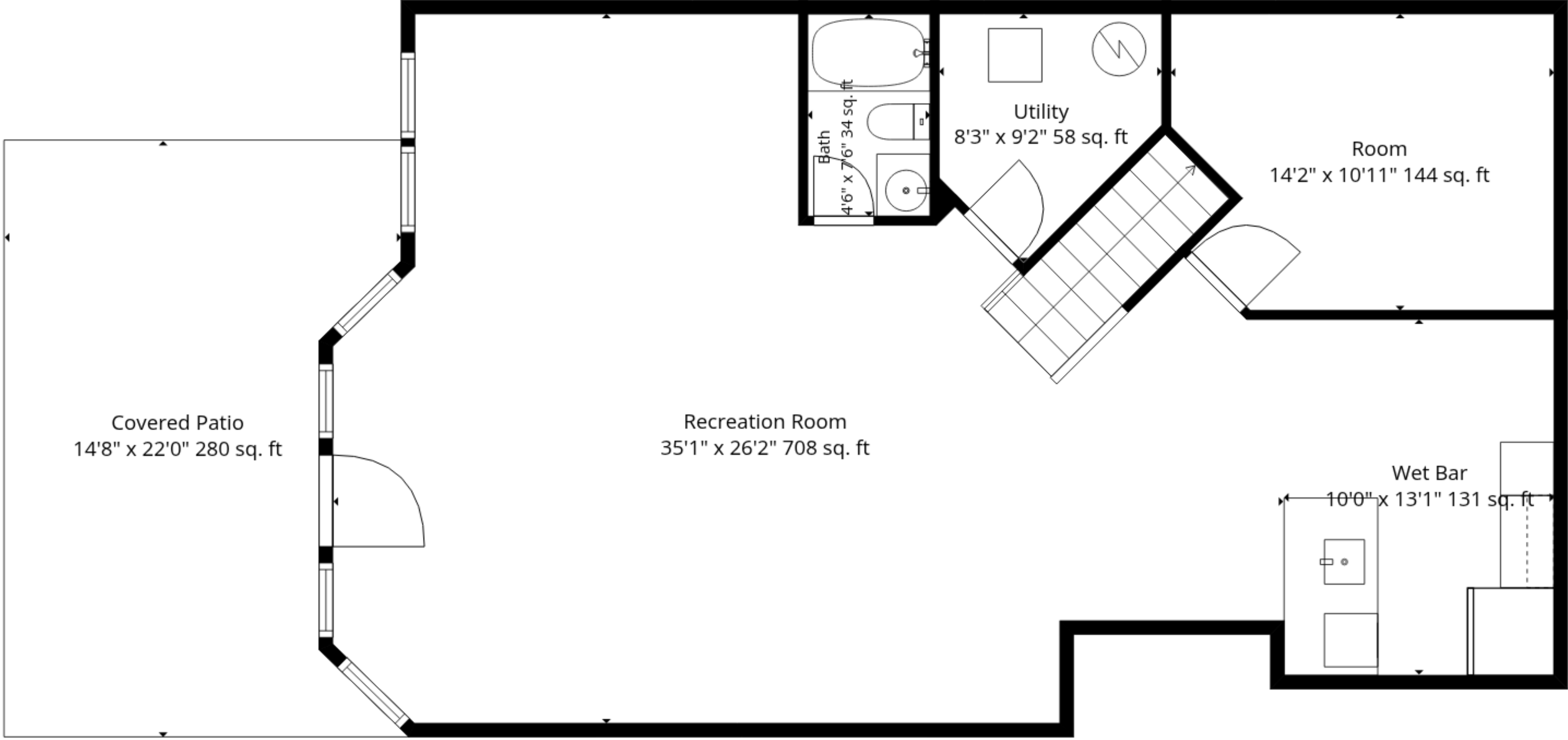
1st Floor
