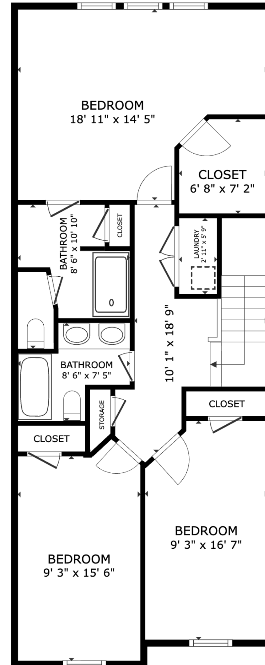
FLOOR 2
