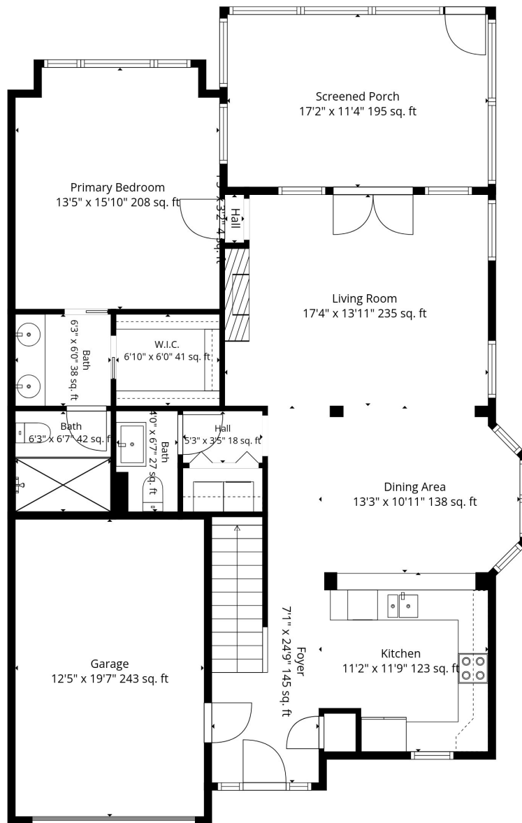
1st Floor
