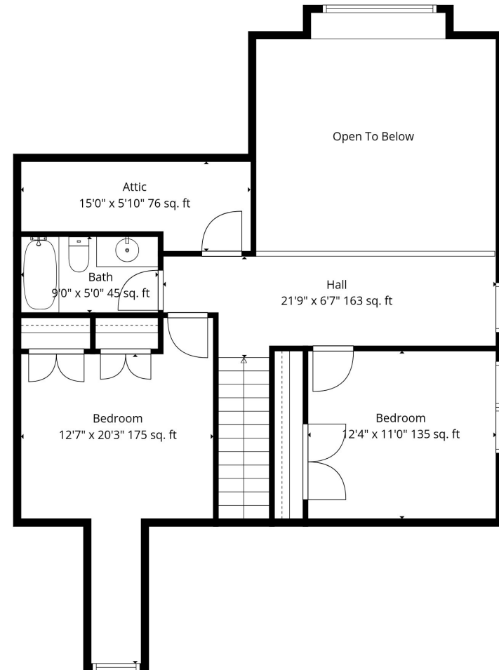
2nd Floor
