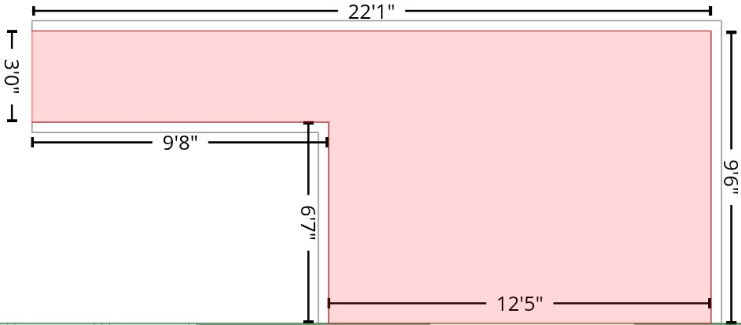
DECK (3) [AREA: 147]
