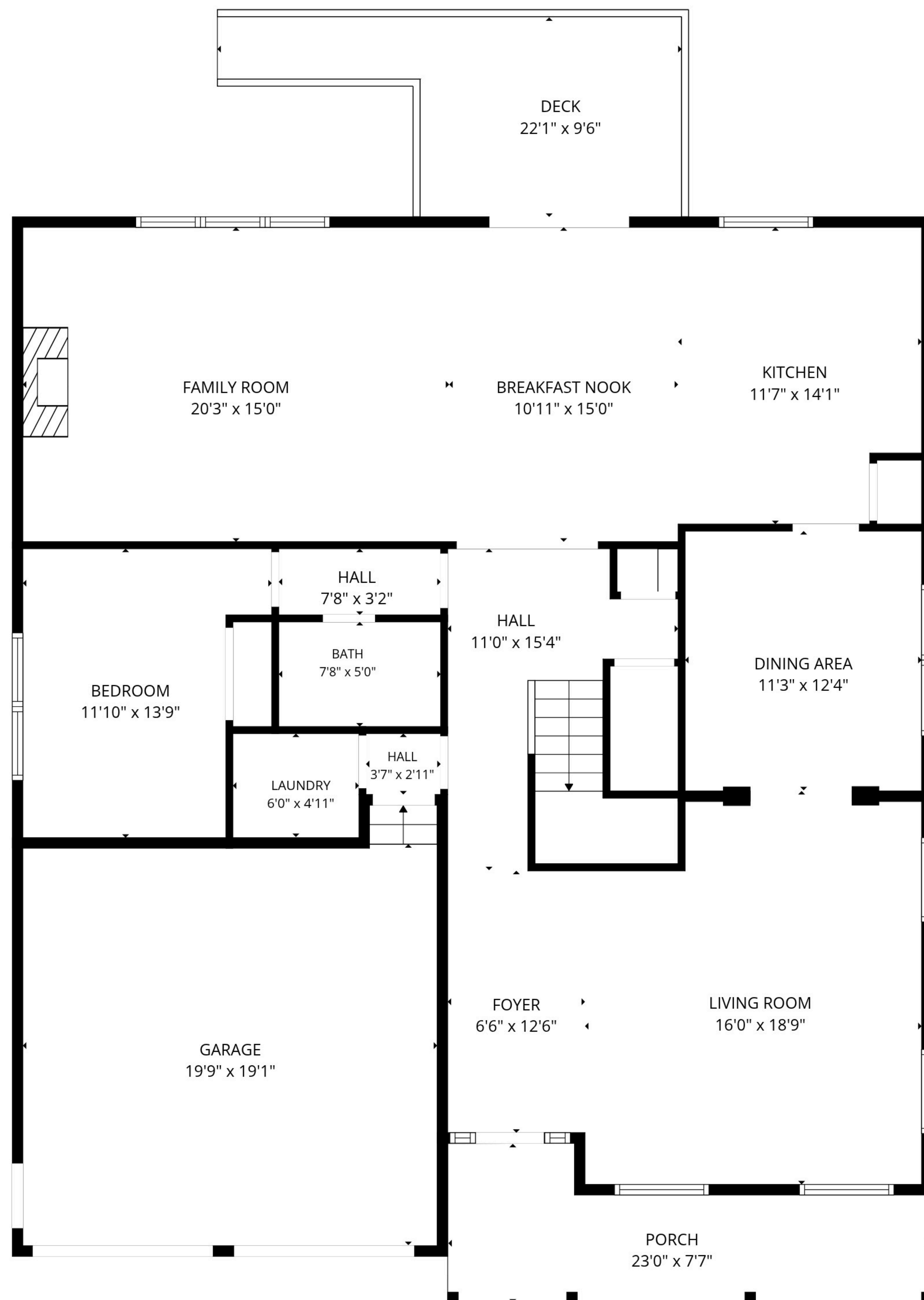
1st floor
