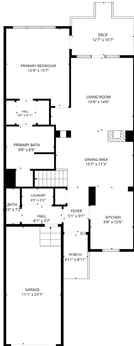
1st floor
