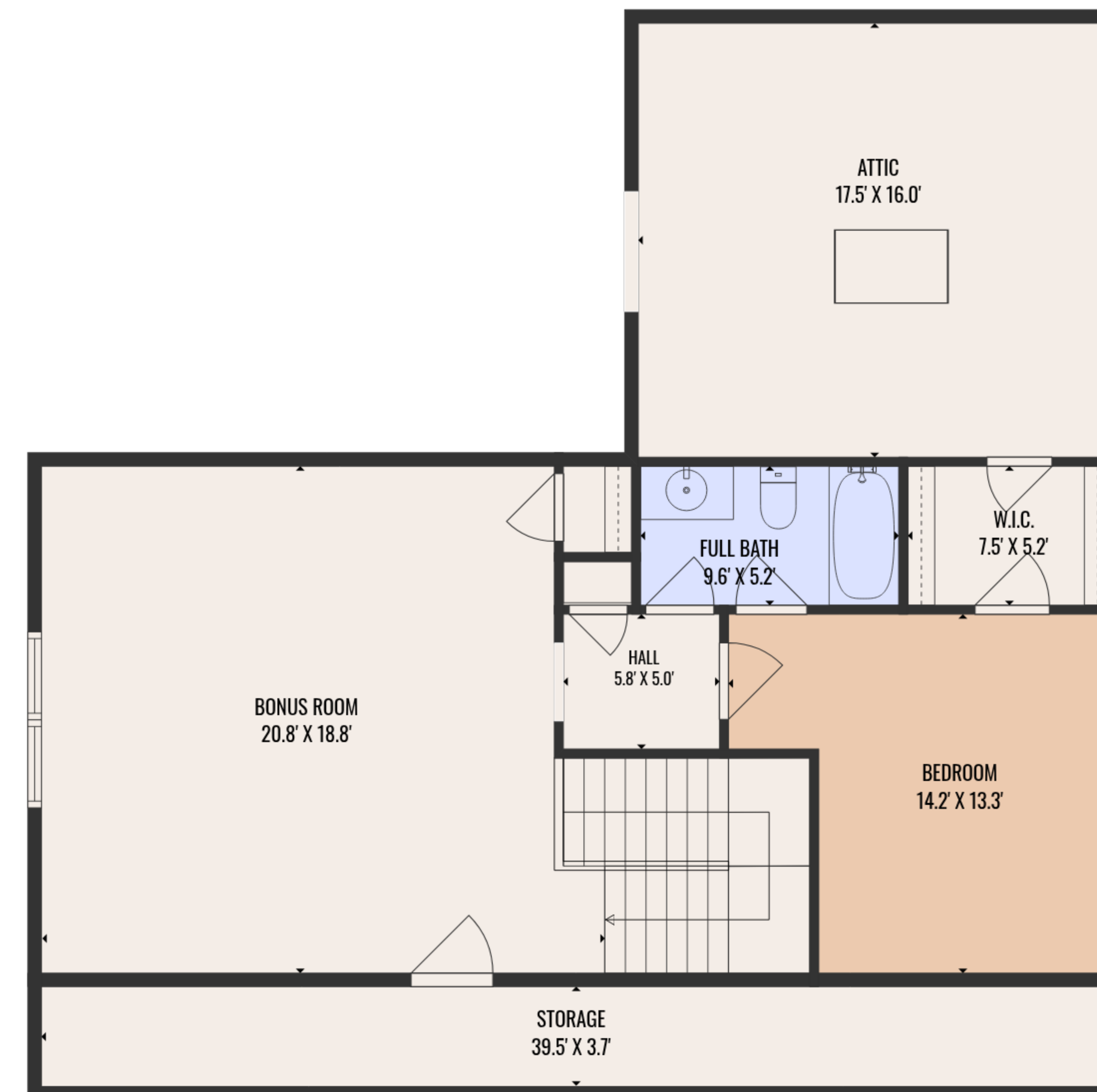
2ND FLOOR
