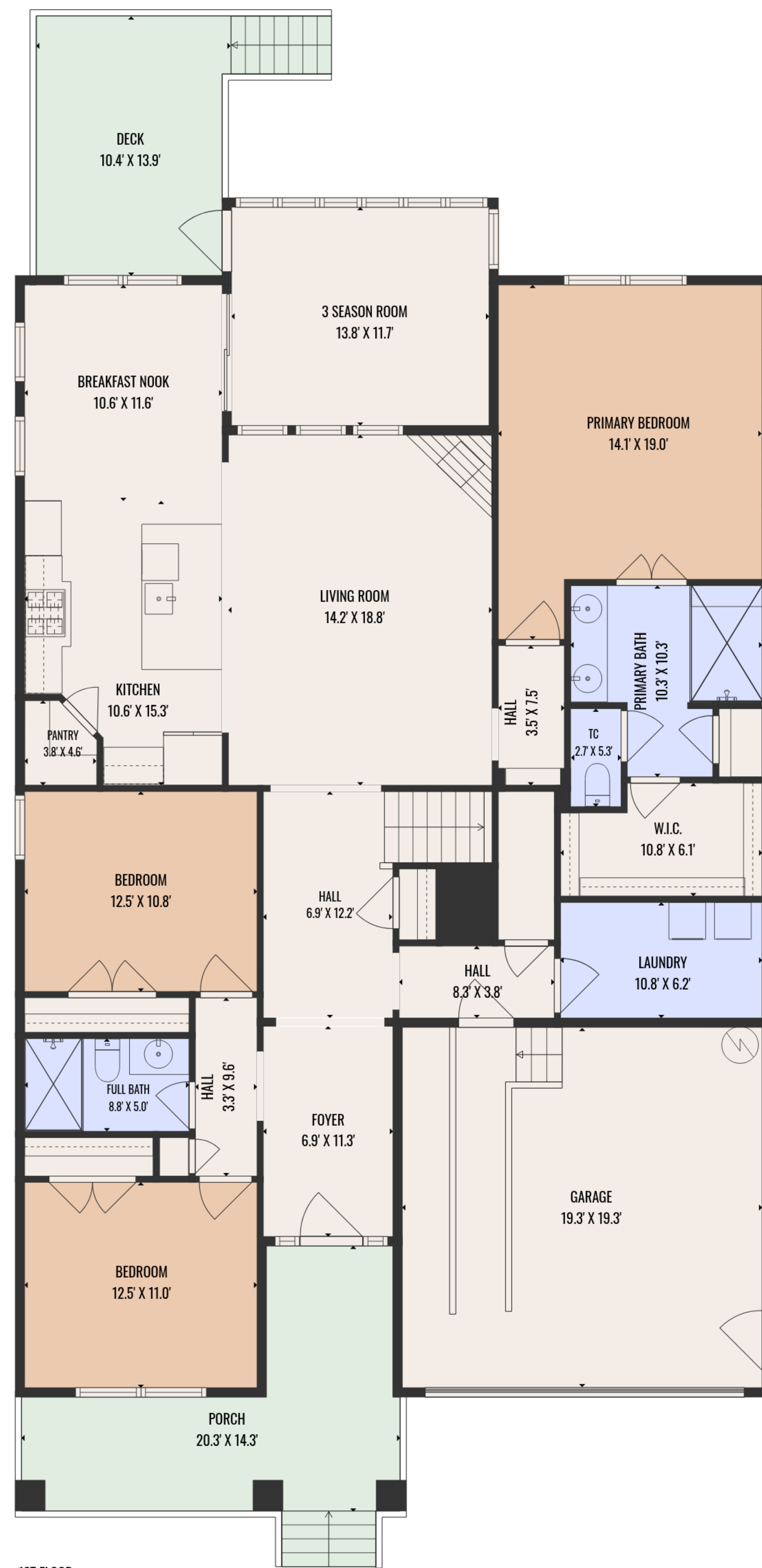
1ST FLOOR
