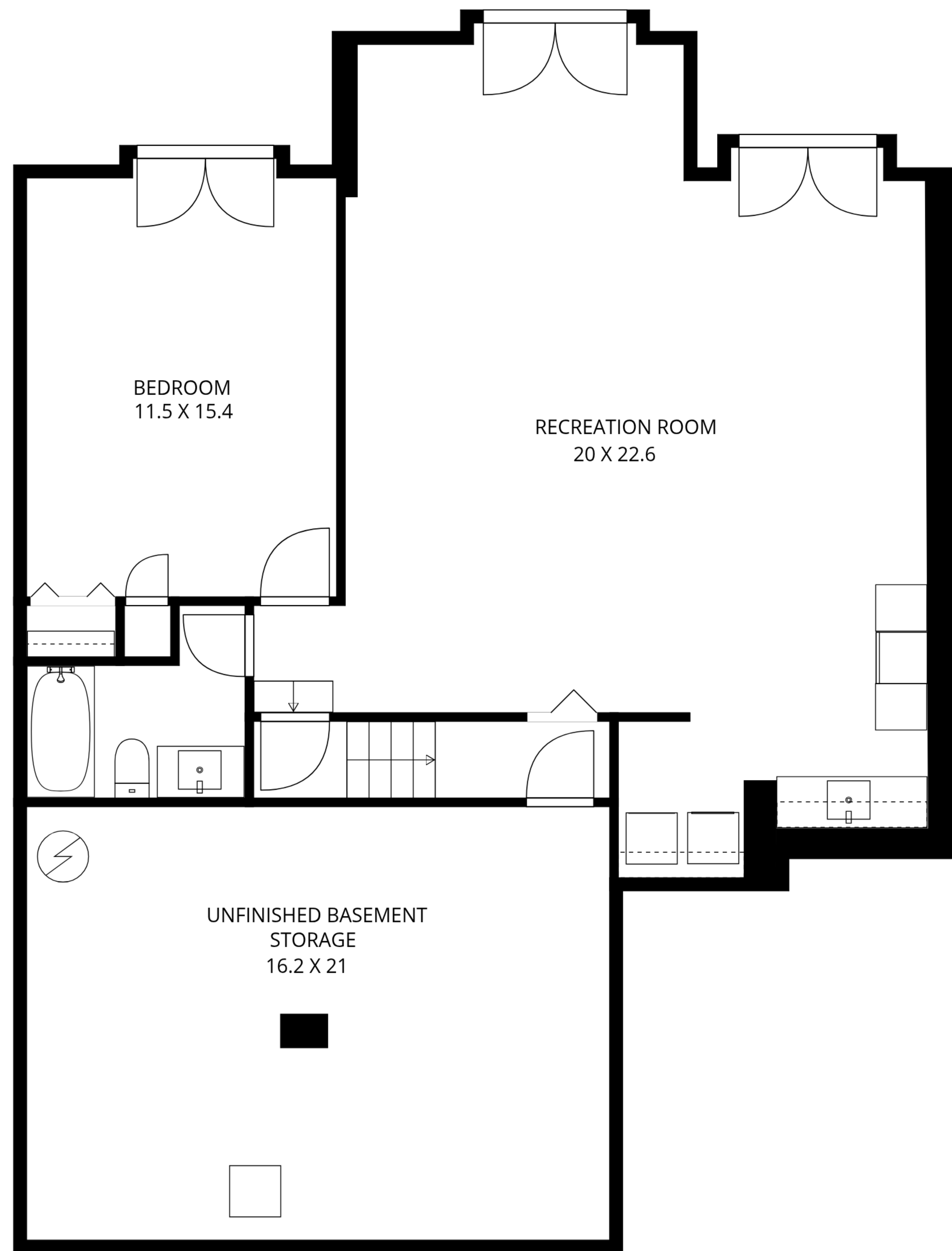
BASEMENT
