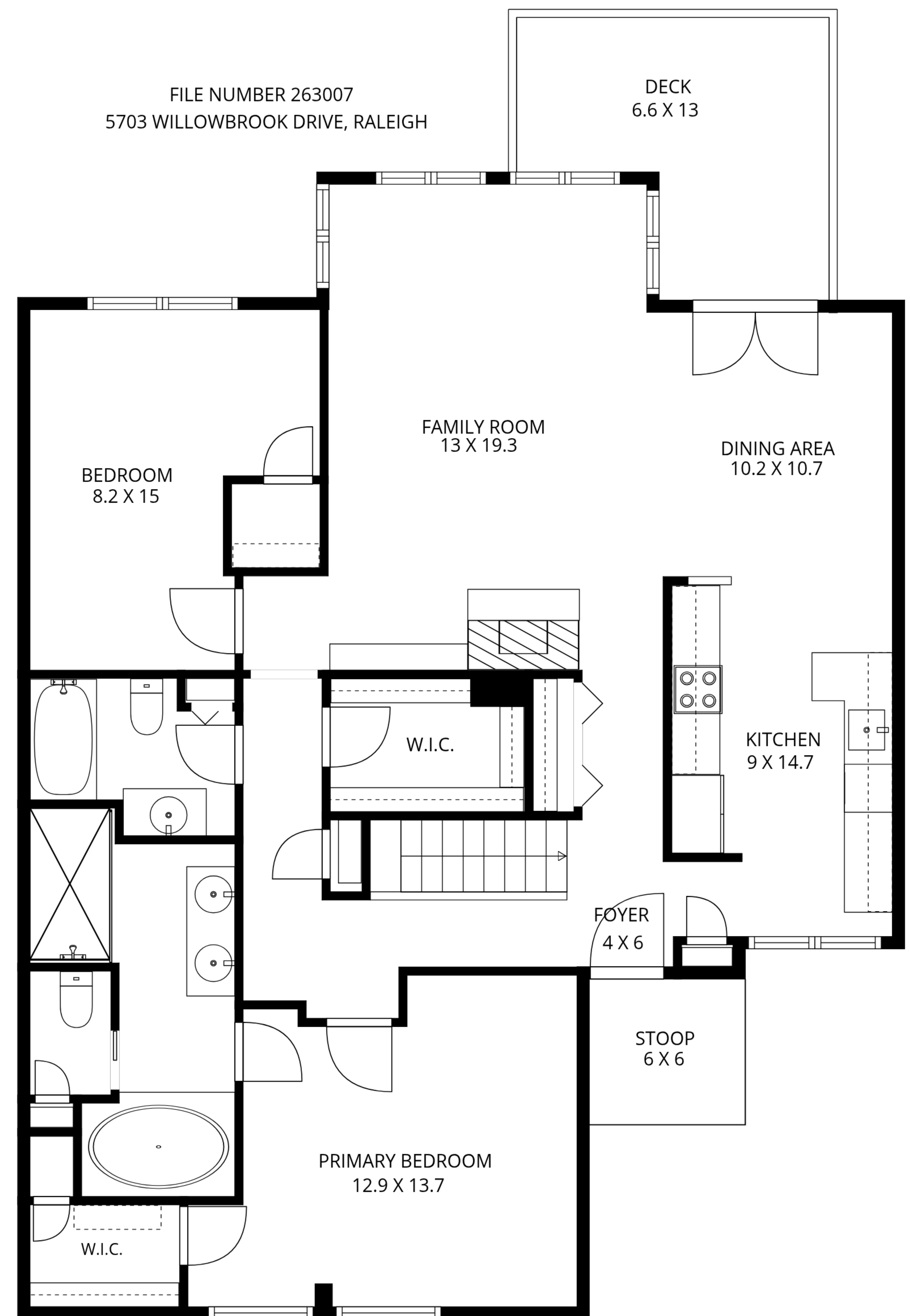
1ST FLOOR
