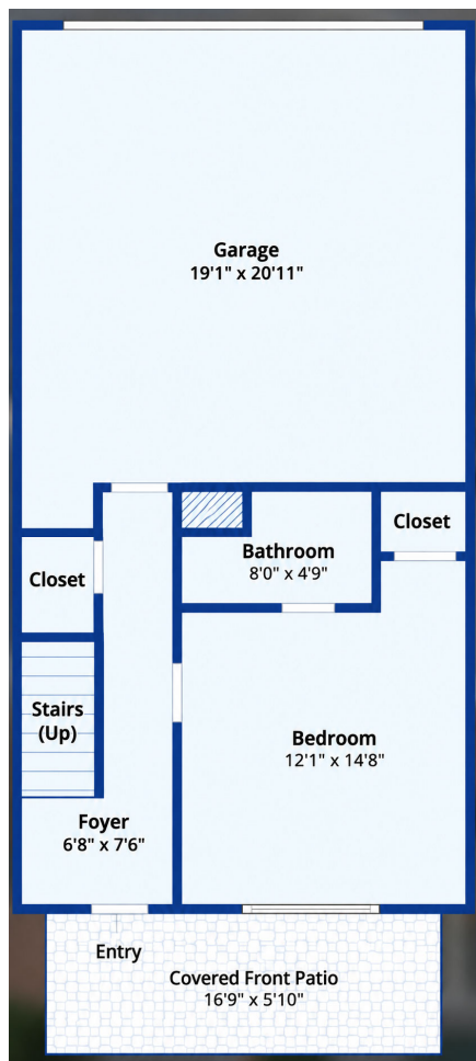
First Floor
