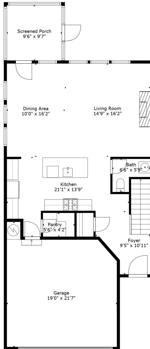
Floor 1
