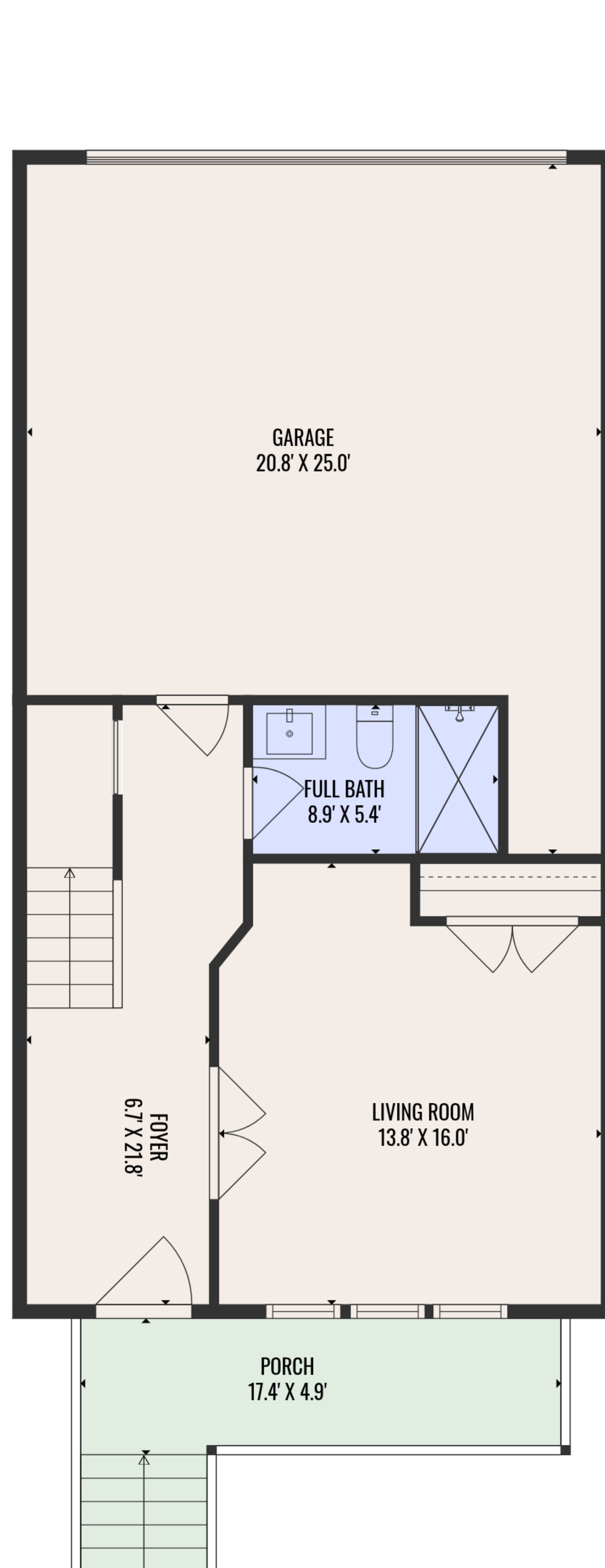
1ST FLOOR
