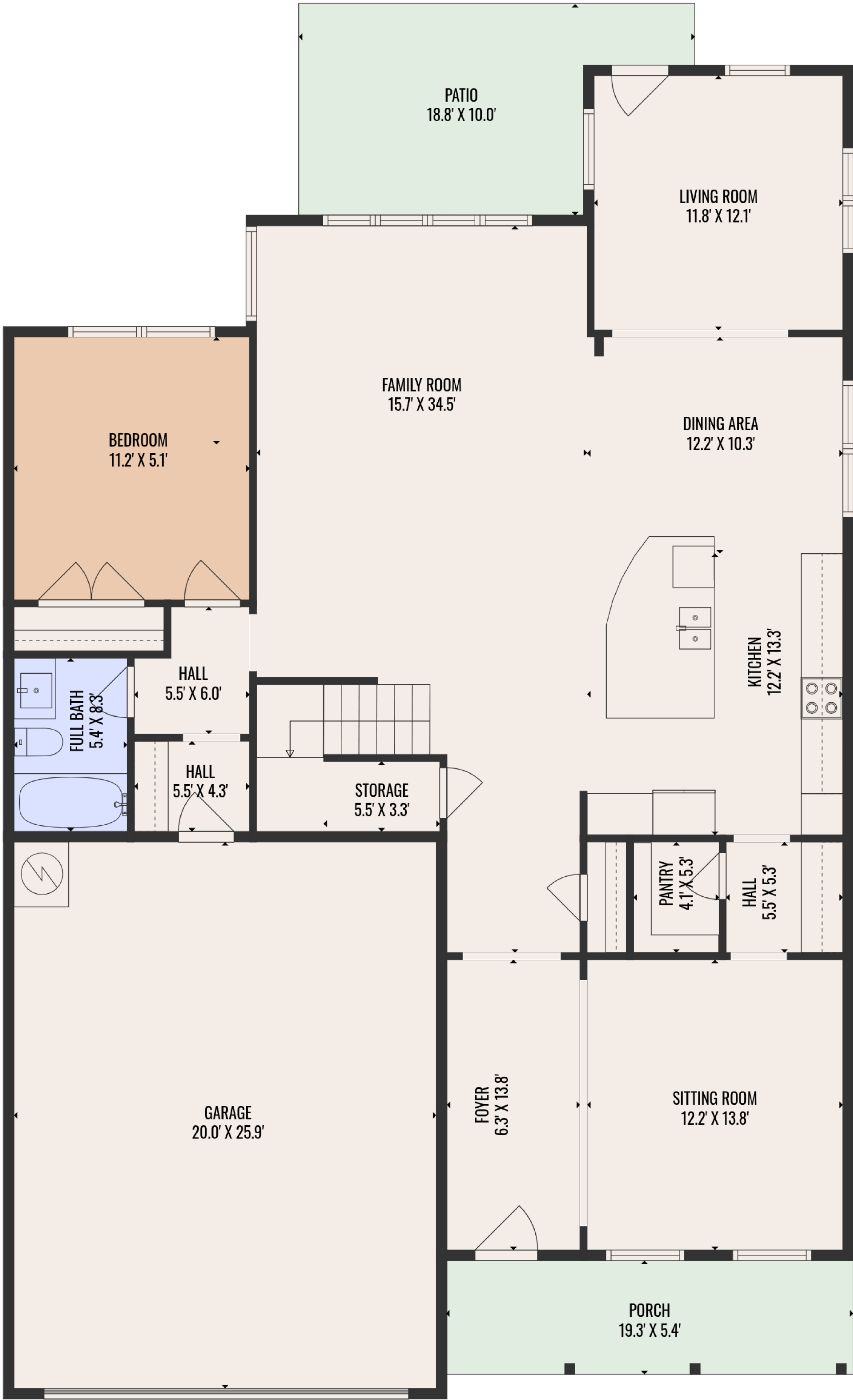
1ST FLOOR
