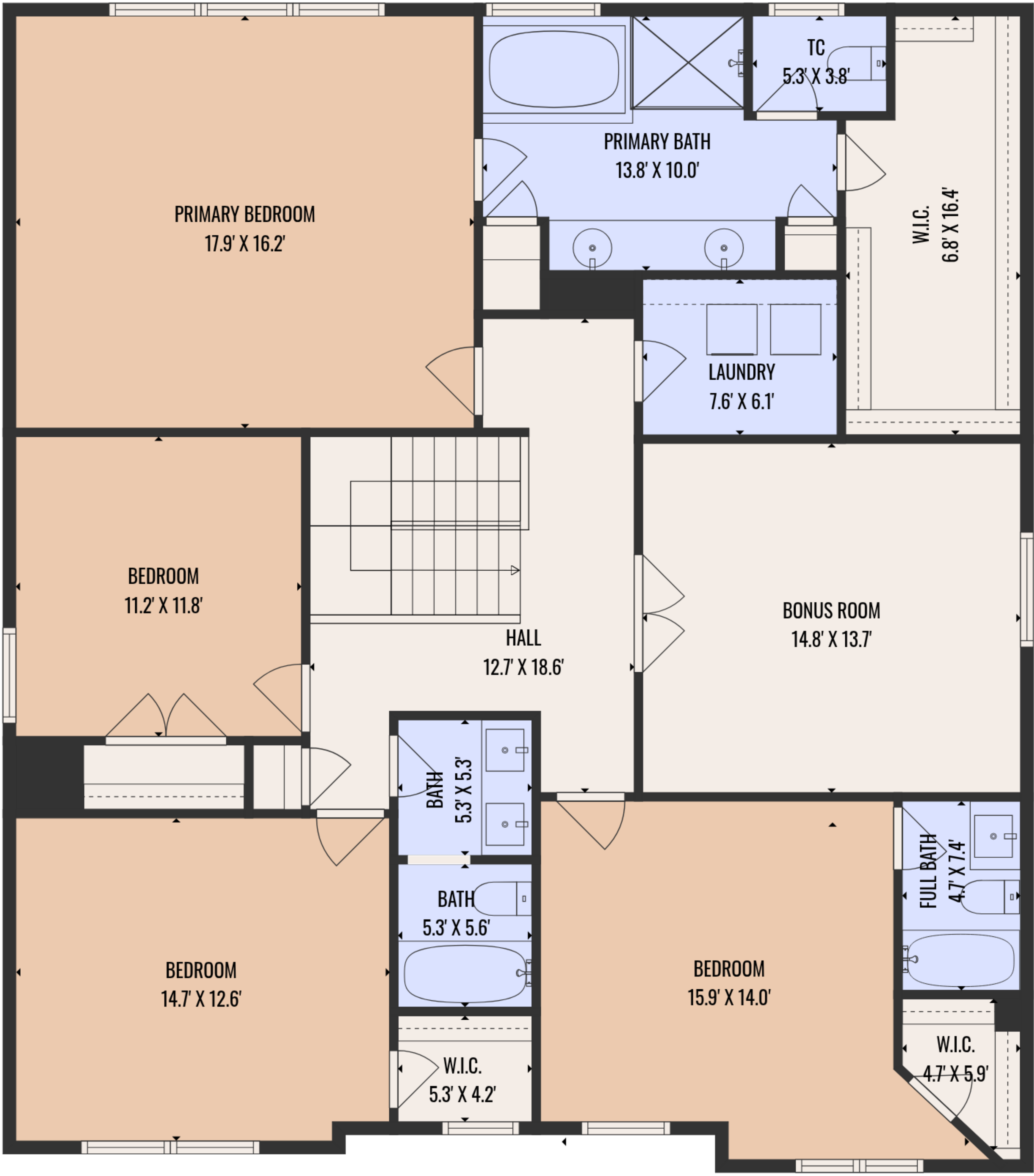
2ND FLOOR
