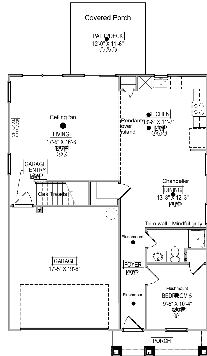
FIRST FLOOR PLAN - B,D
