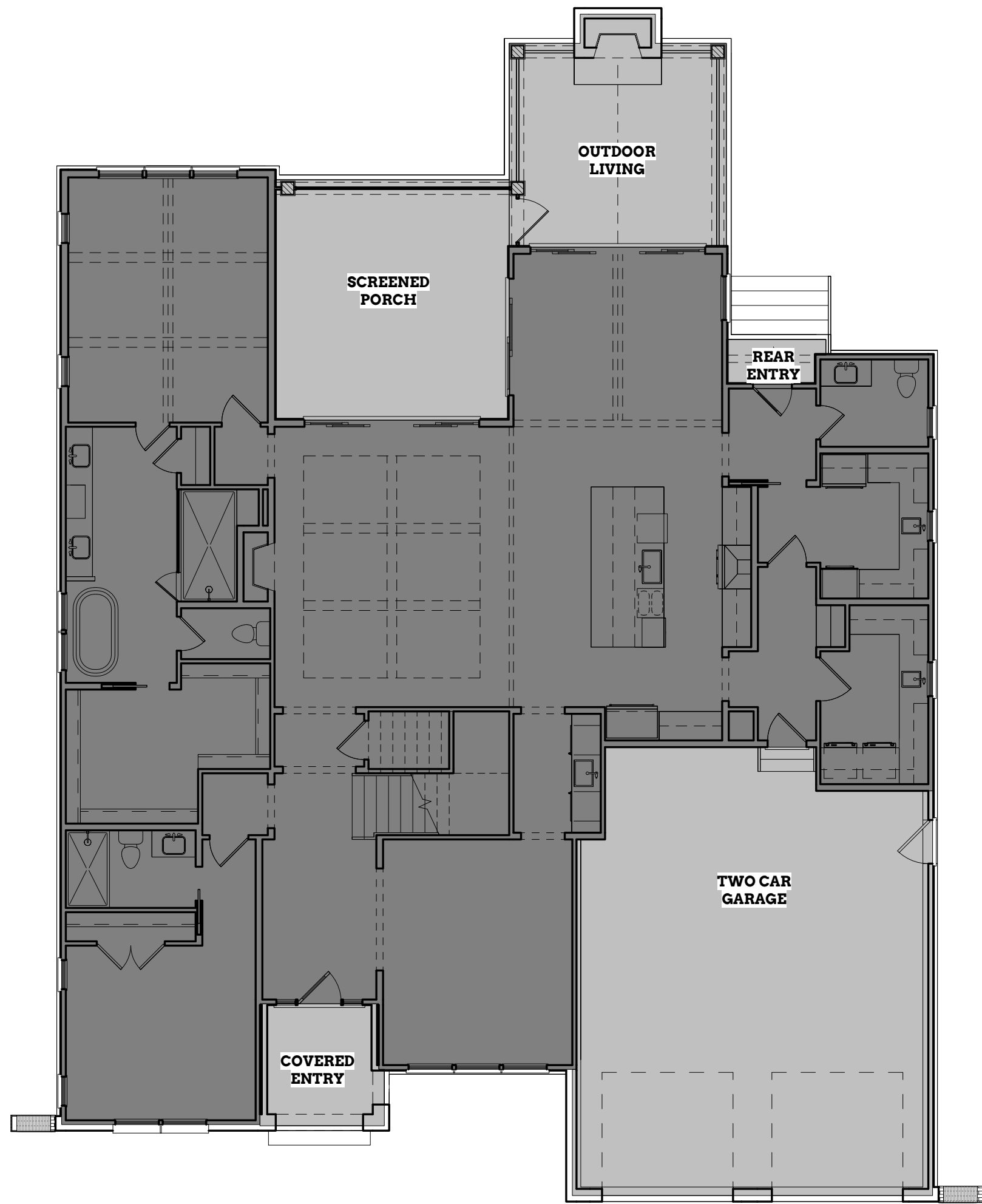
1 First Floor Square Footage A002 1/8" = 1'-0"
