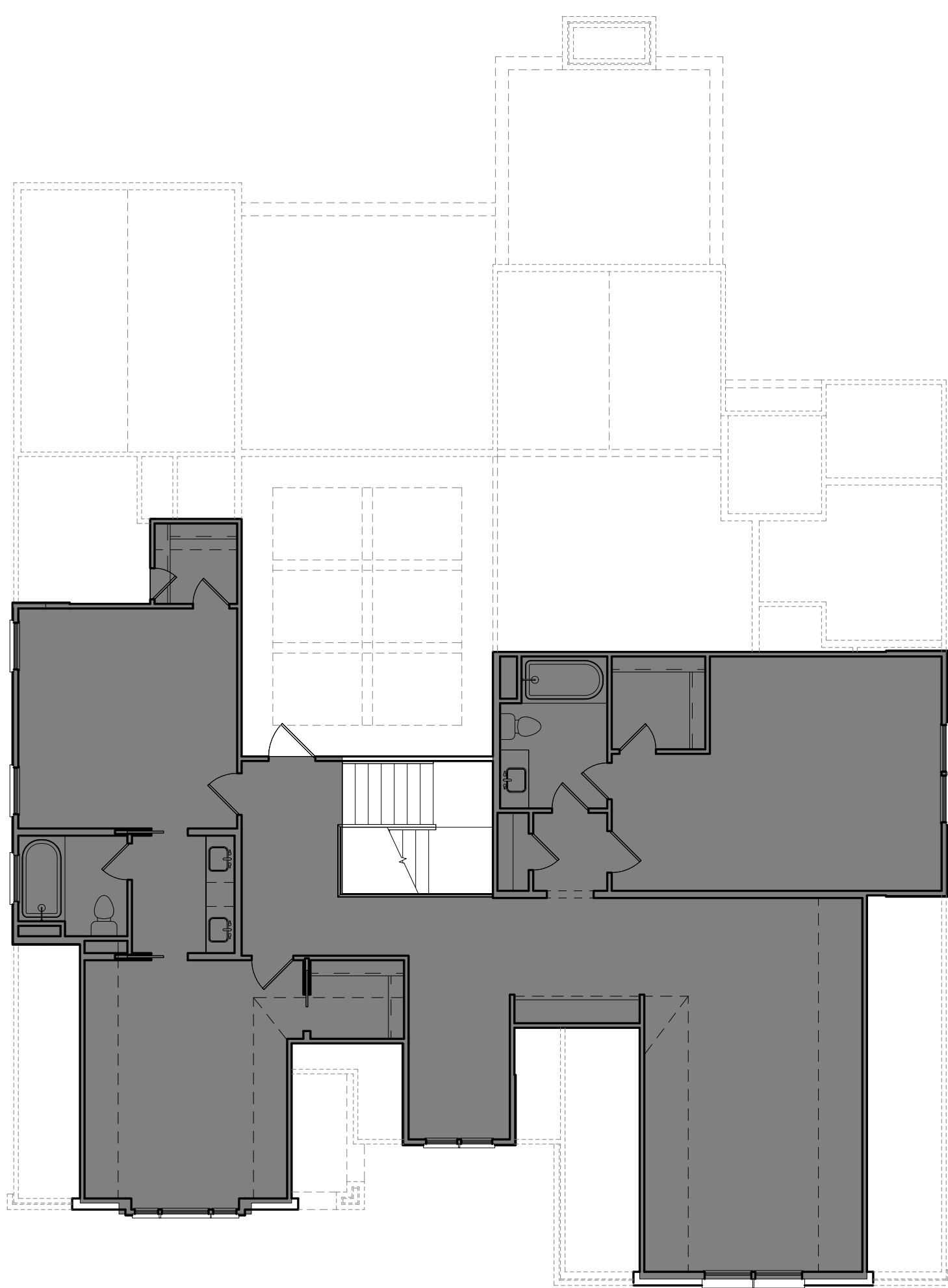
2 Second Floor Square Footage A002 1/8" = 1'-0"
