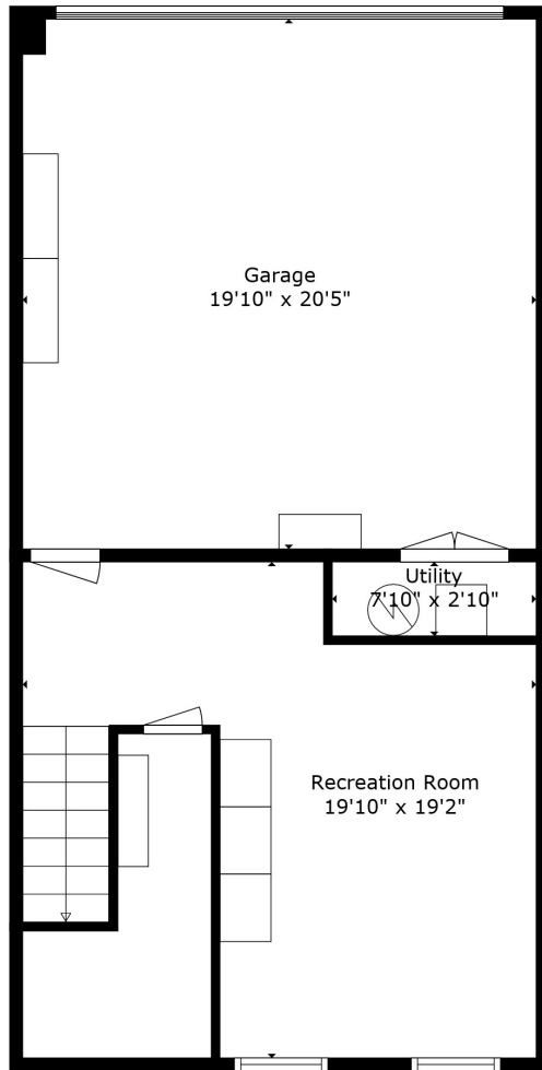
Floor 1
