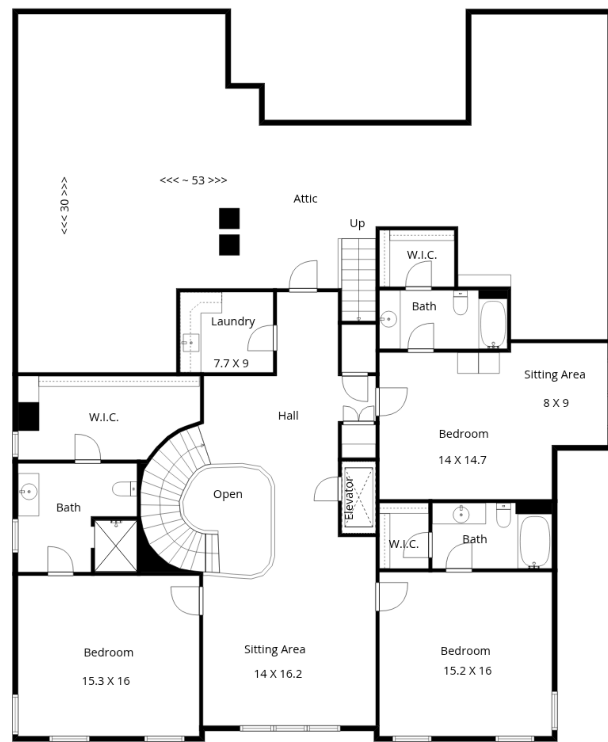
2nd Floor
