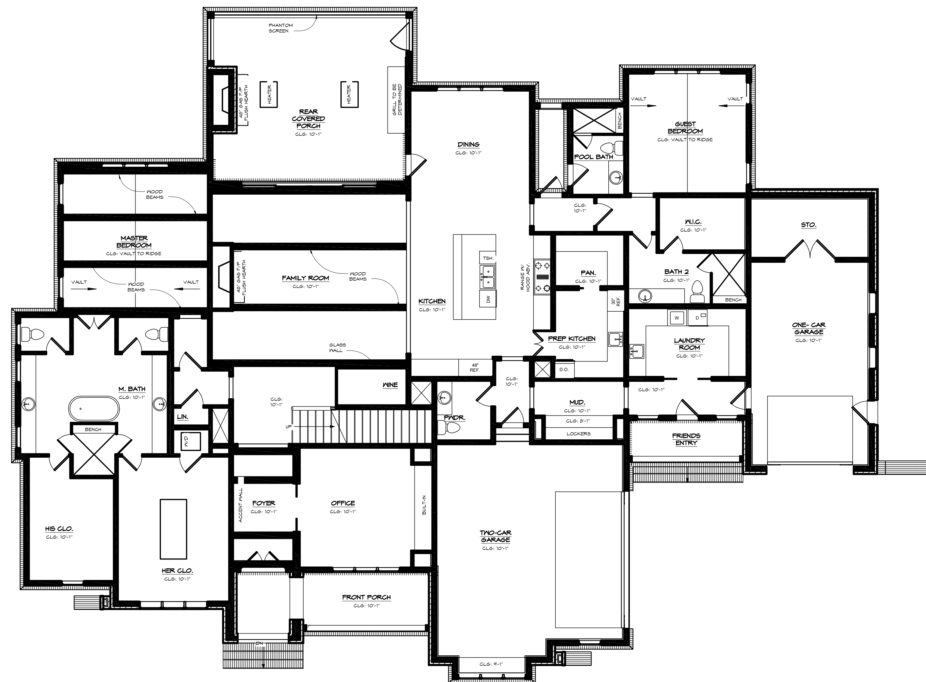
MAIN LEVEL
