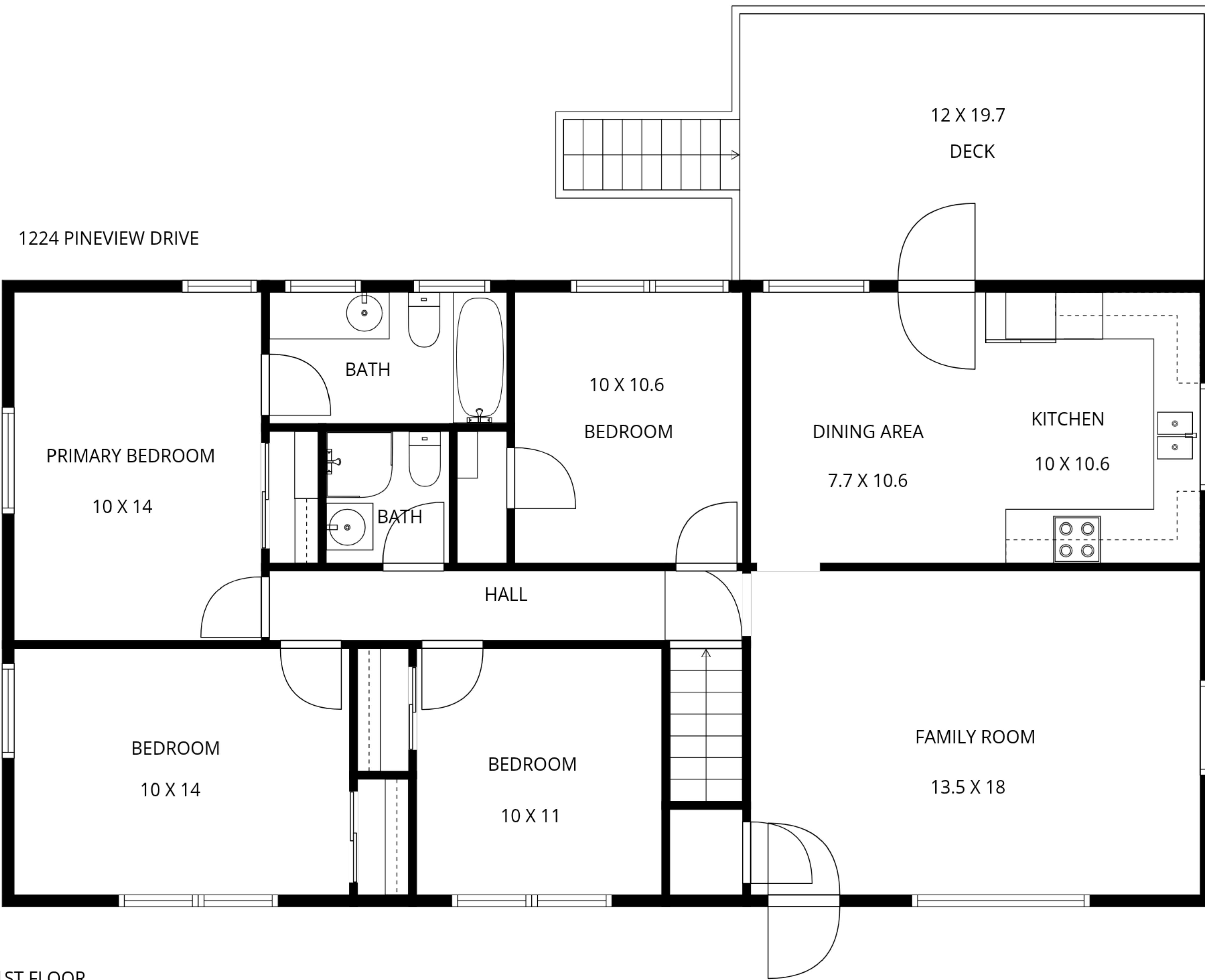
1ST FLOOR
