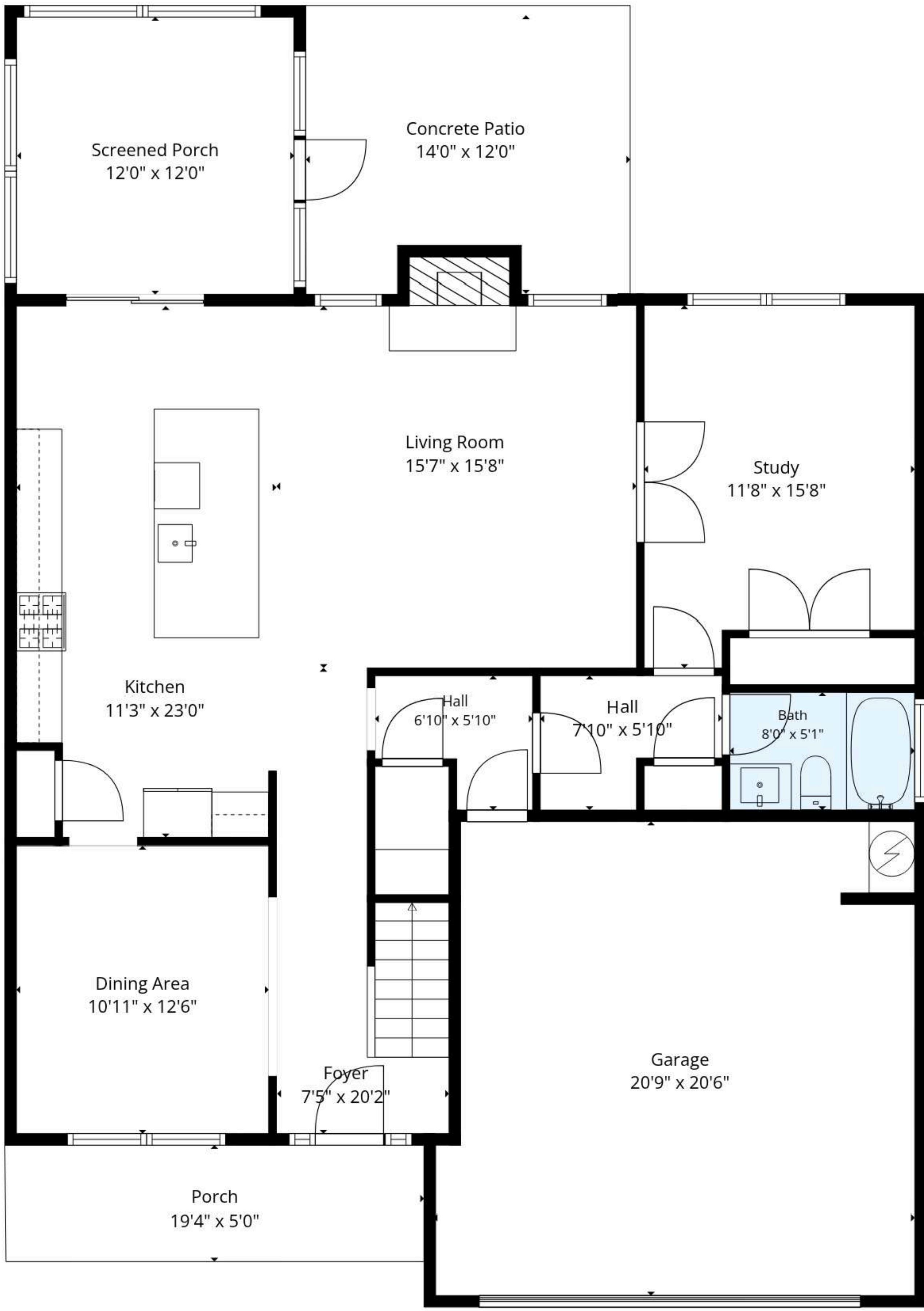
1st Floor
