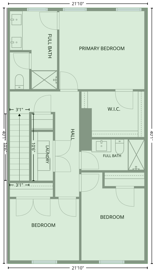
2nd floor [AREA: 874]
