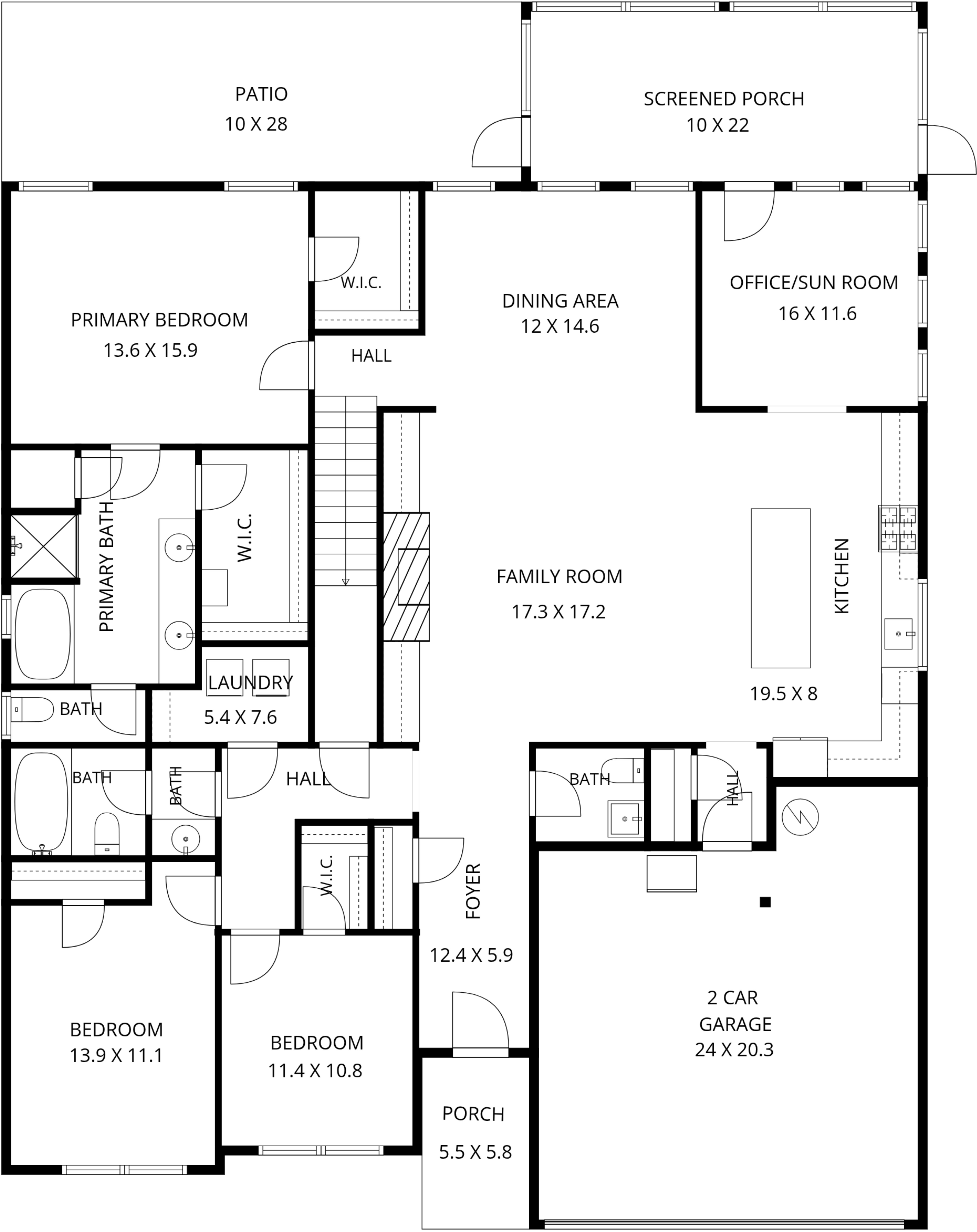
1ST FLOOR
