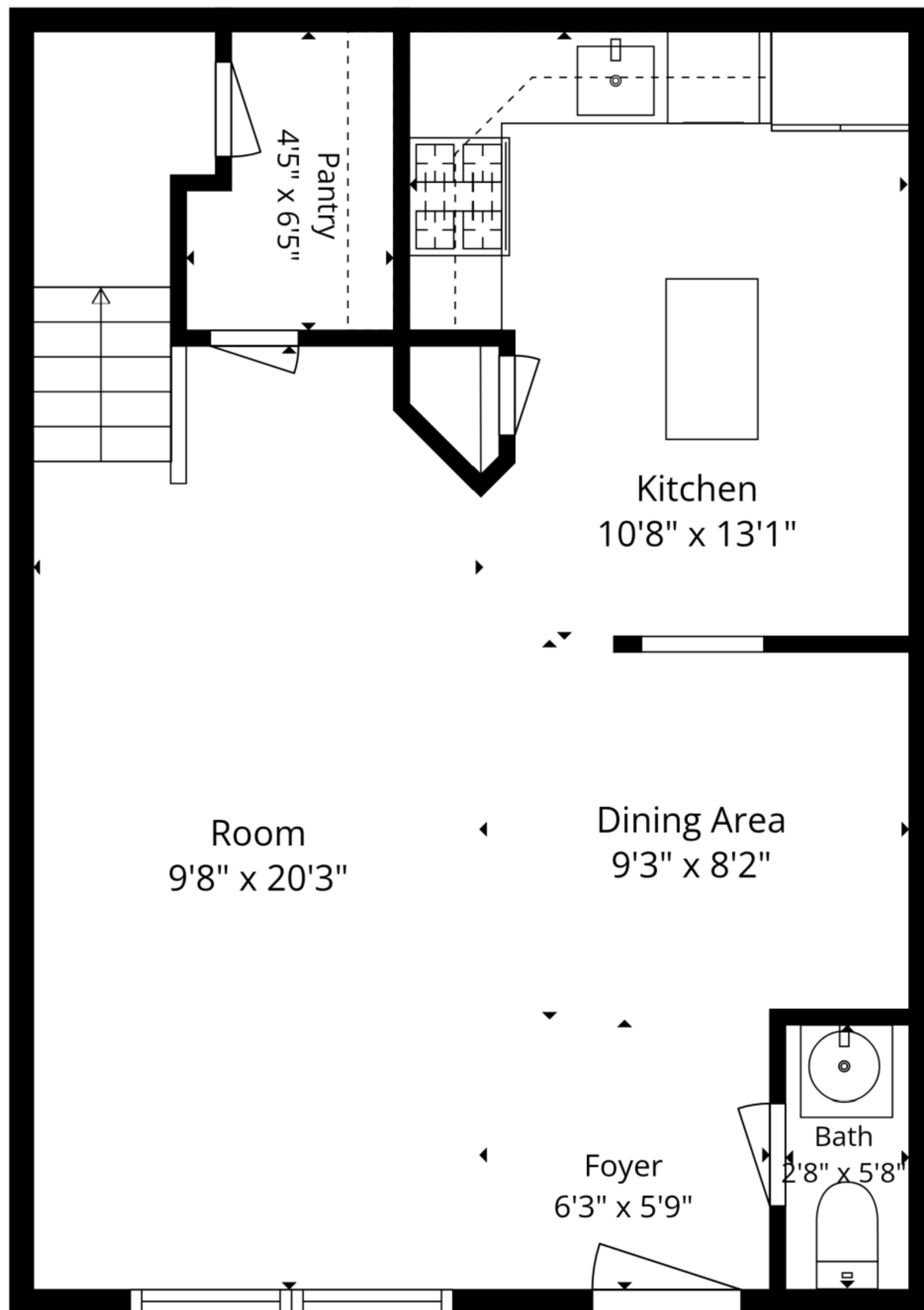
Main Floor
