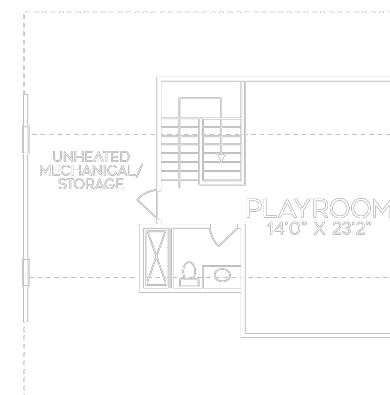
THIRD/ ATTIC FLOOR
