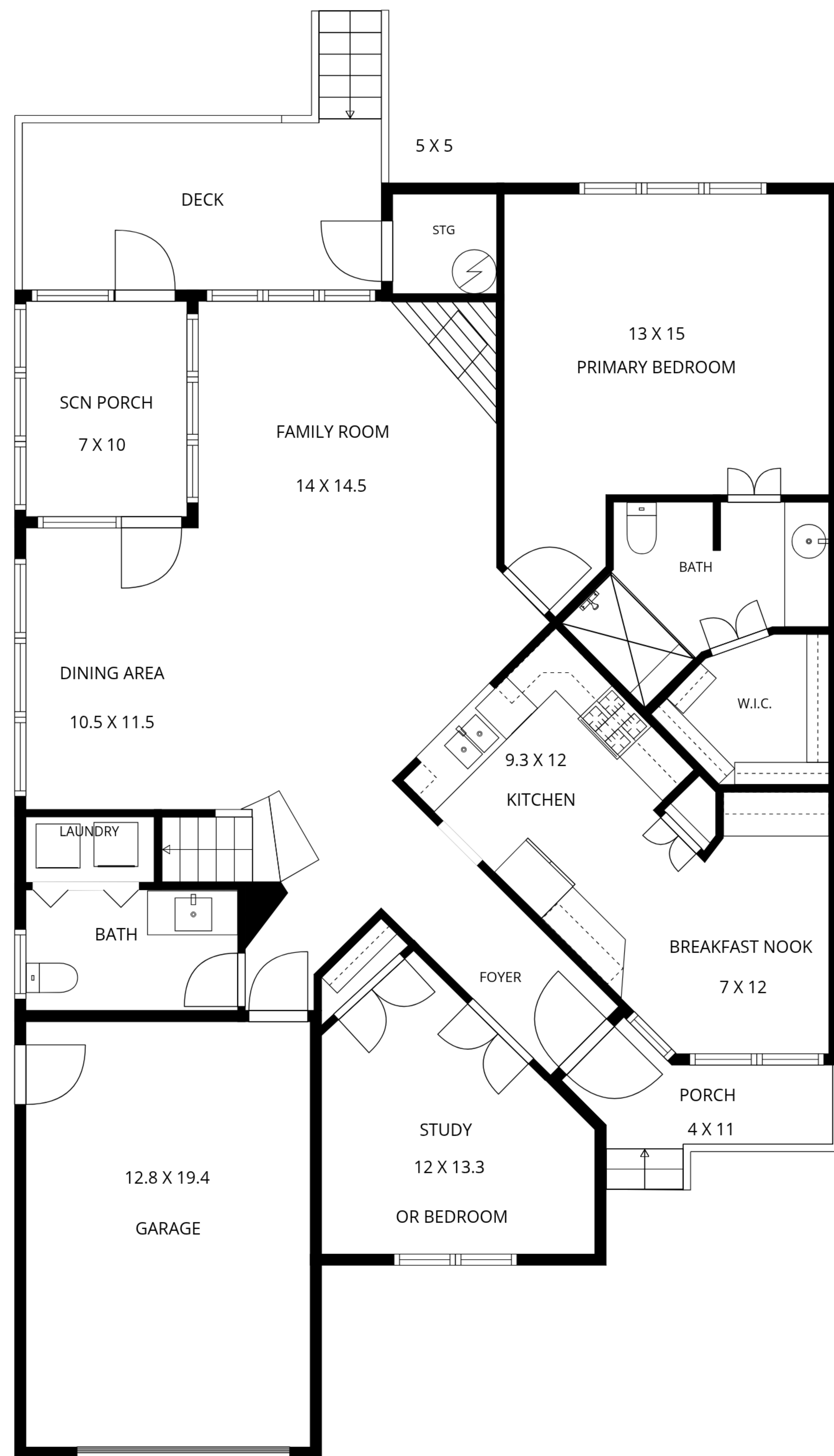
1ST FLOOR
