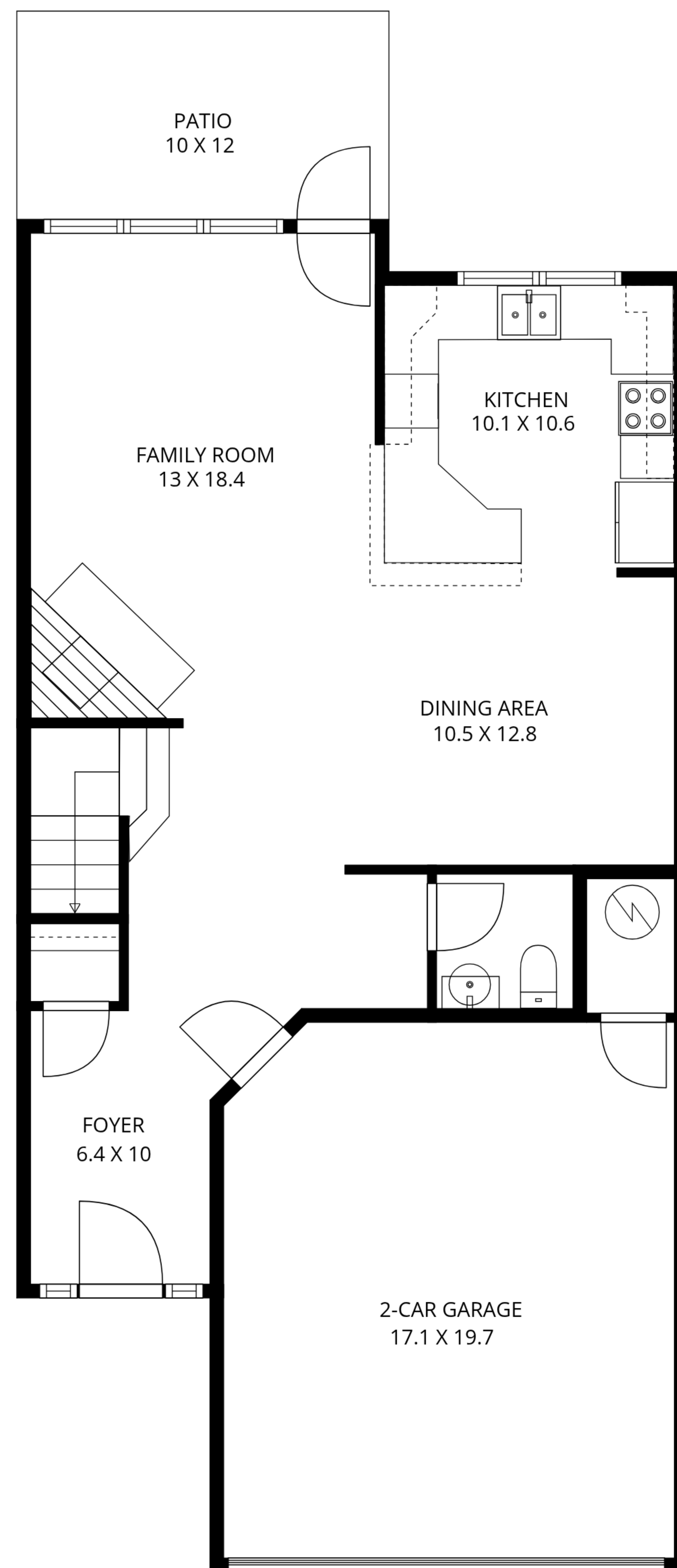
1ST FLOOR
