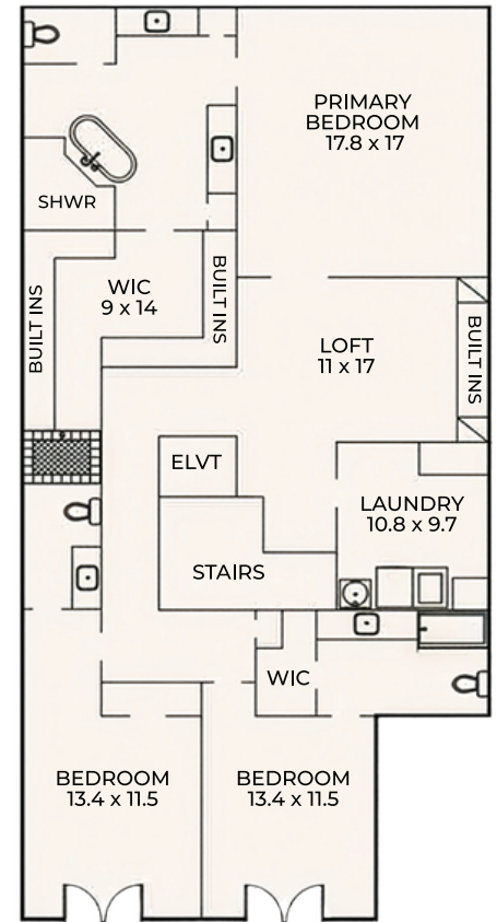
SECOND FLOOR
