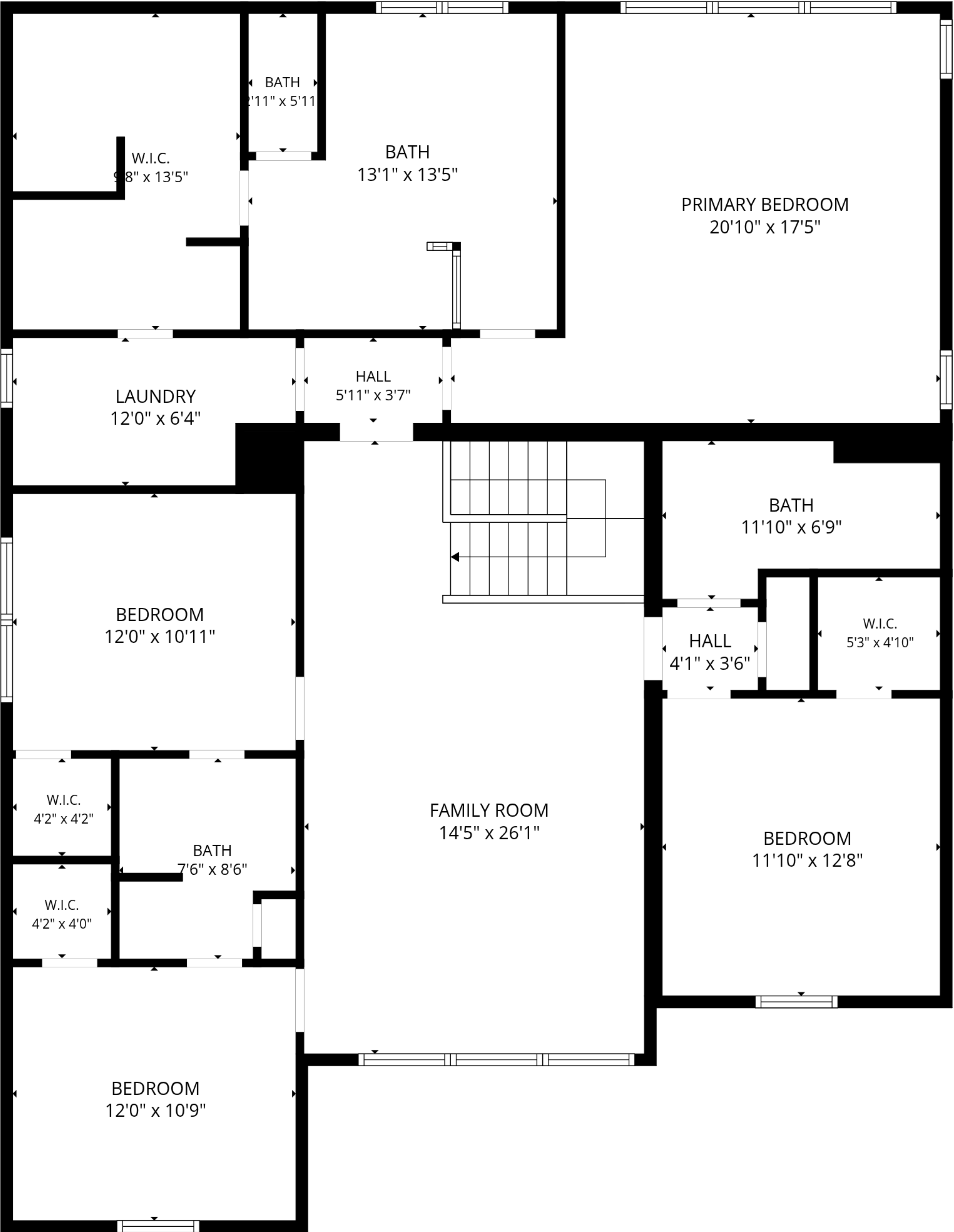
2nd floor
