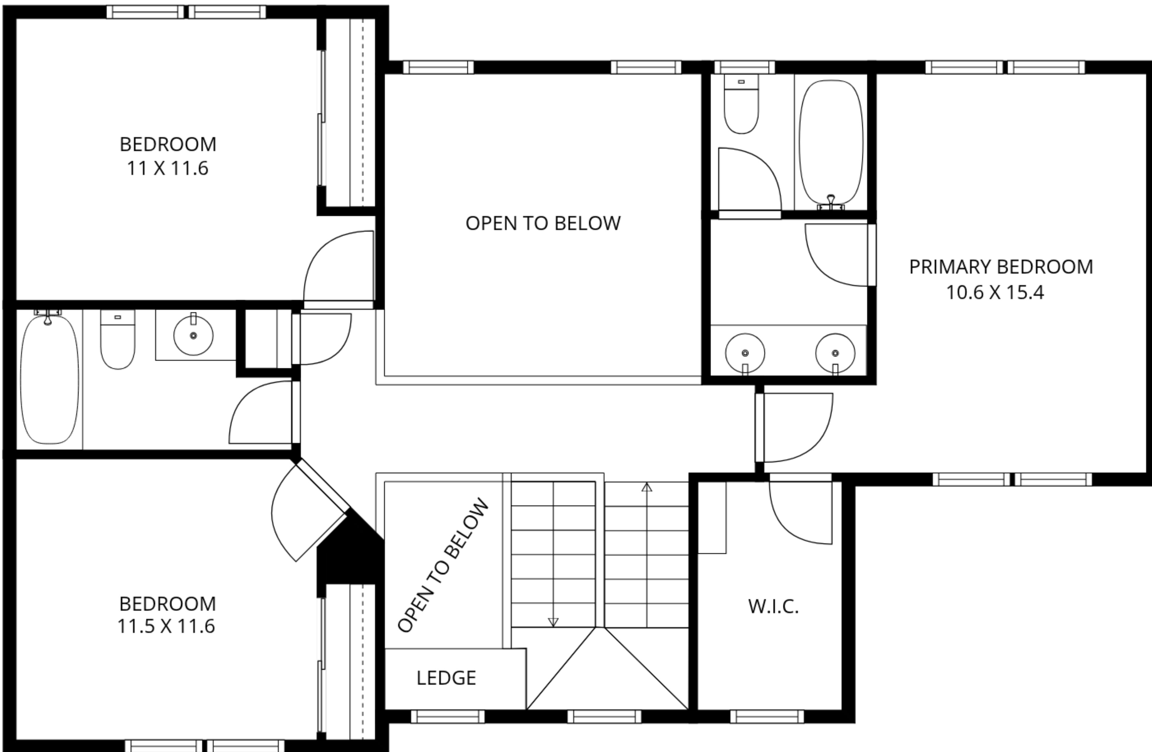
2ND FLOOR
