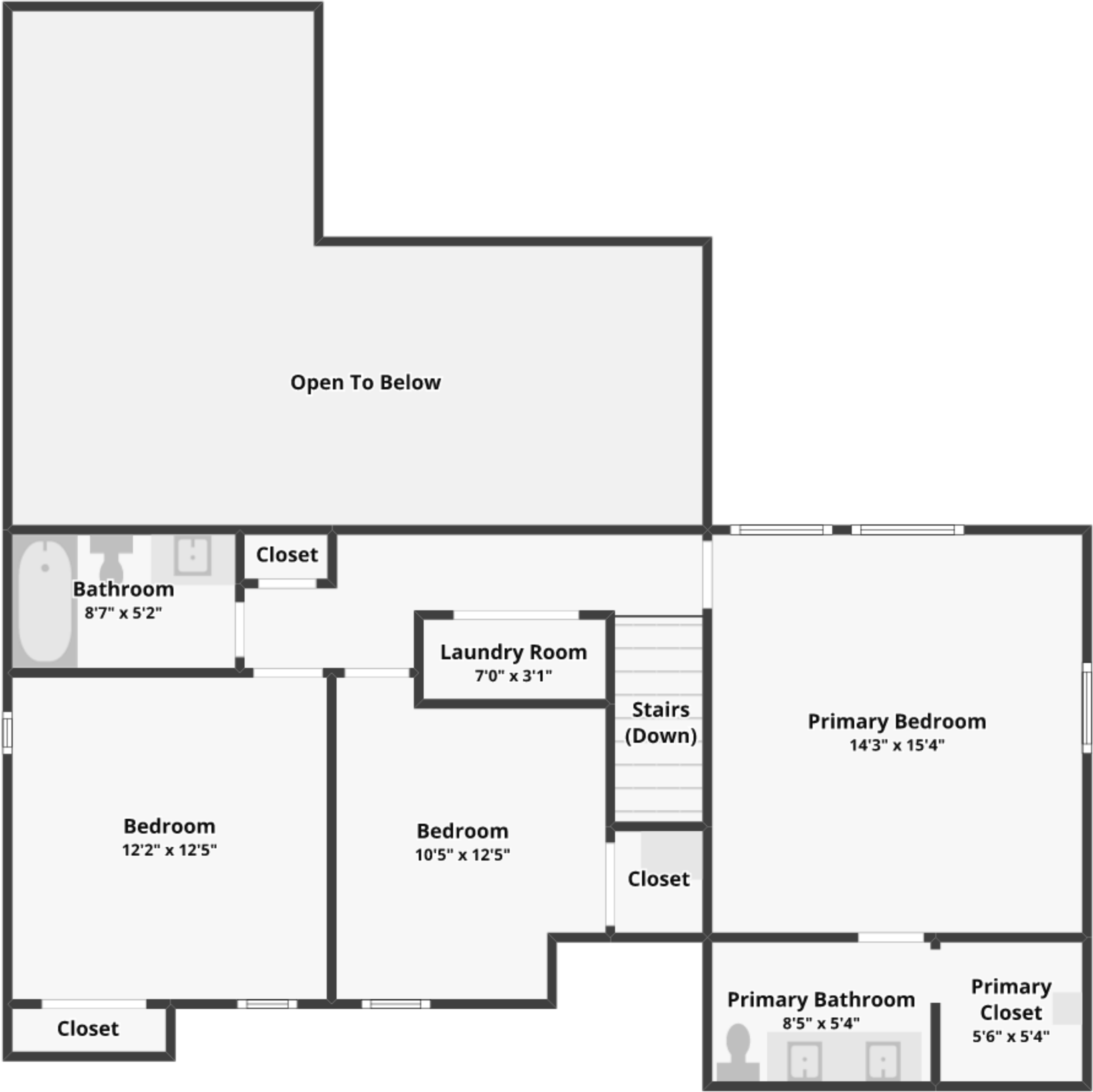
FLOOR 2
