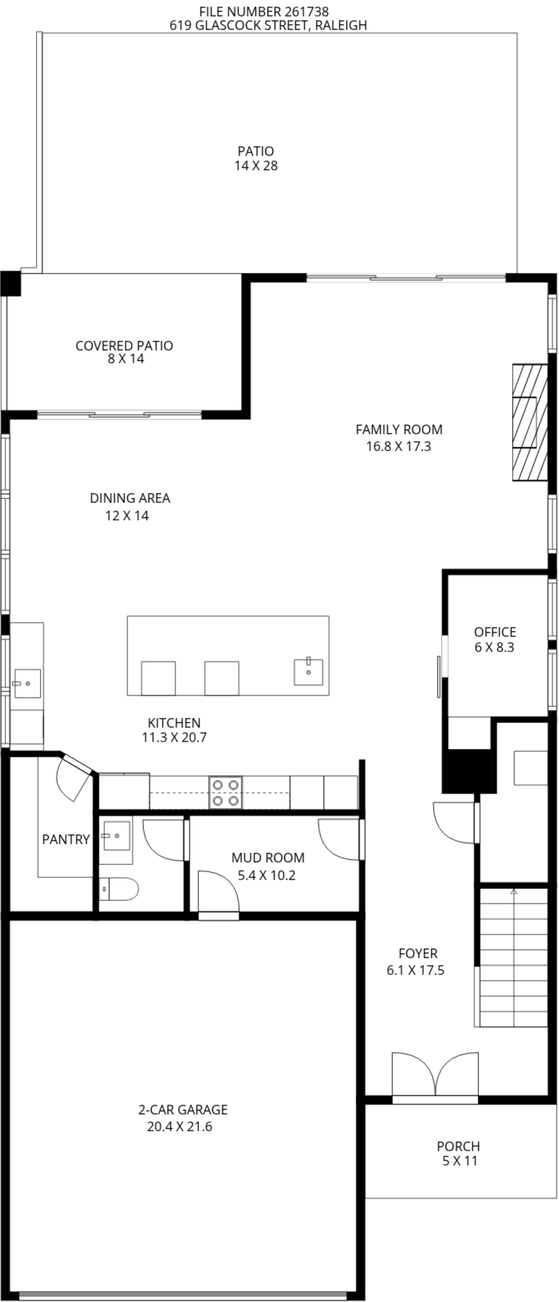
1ST FLOOR
