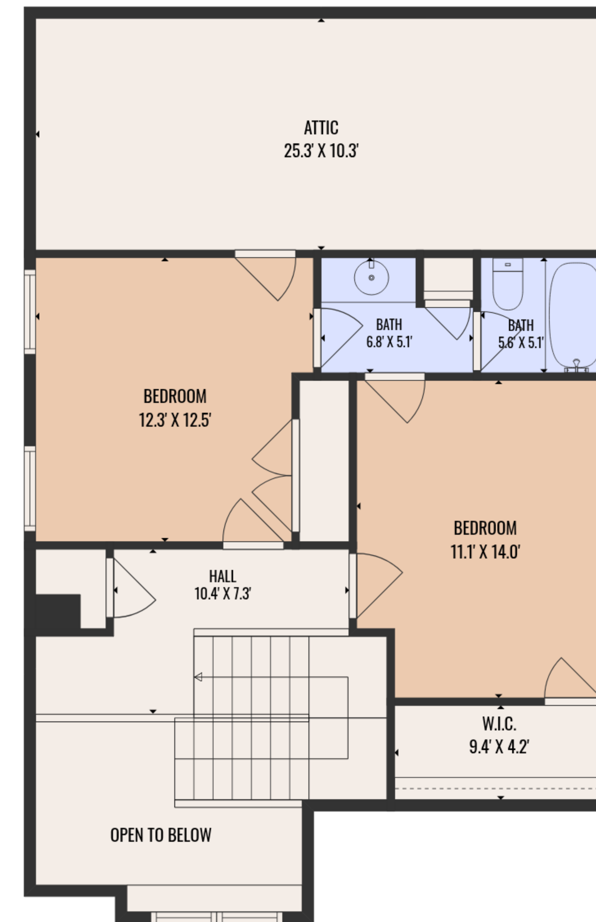
2ND FLOOR
