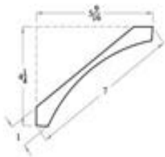
EC81 CROWN ROUND SHOE MOULDING
