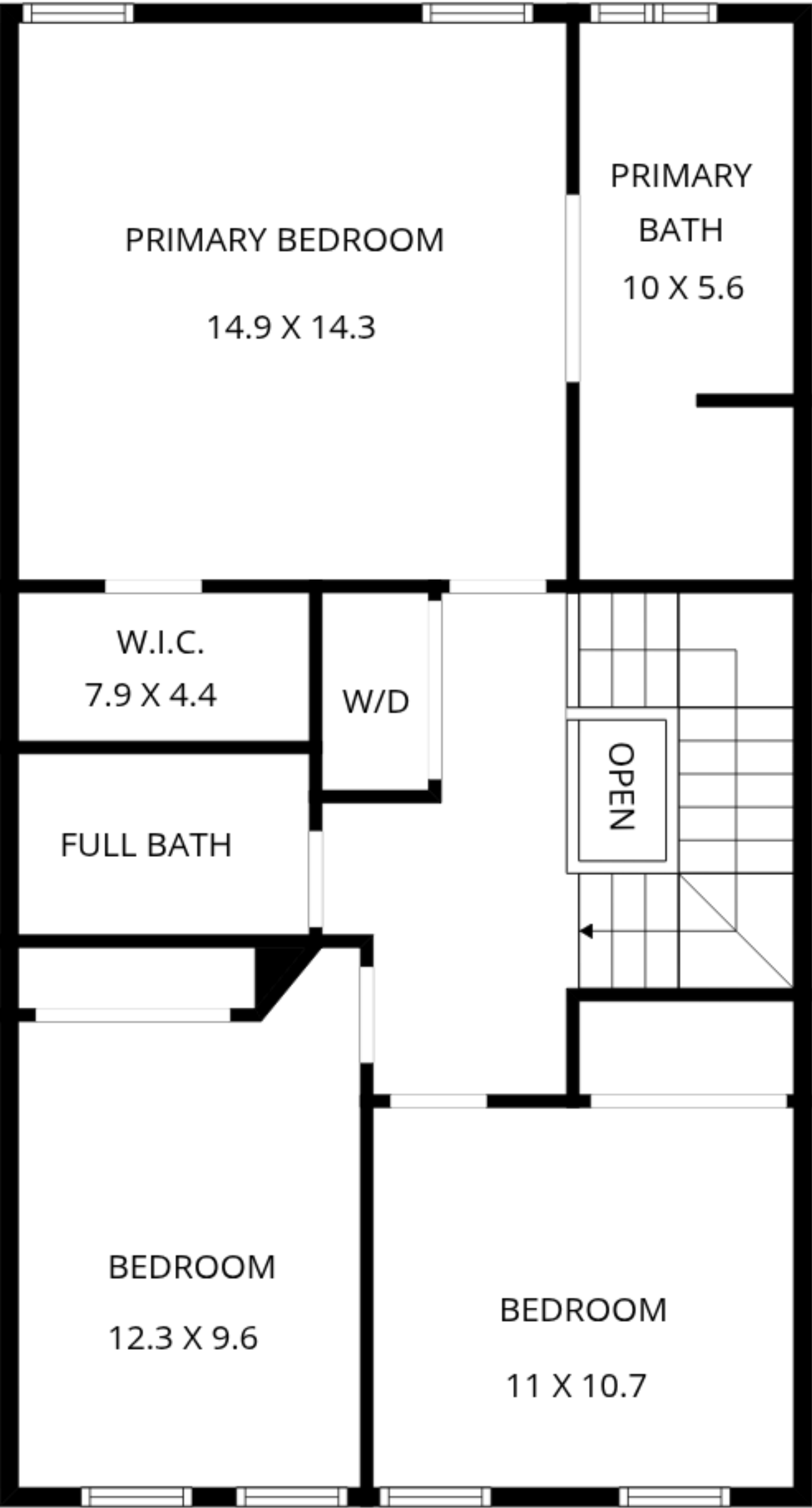
3rd floor
