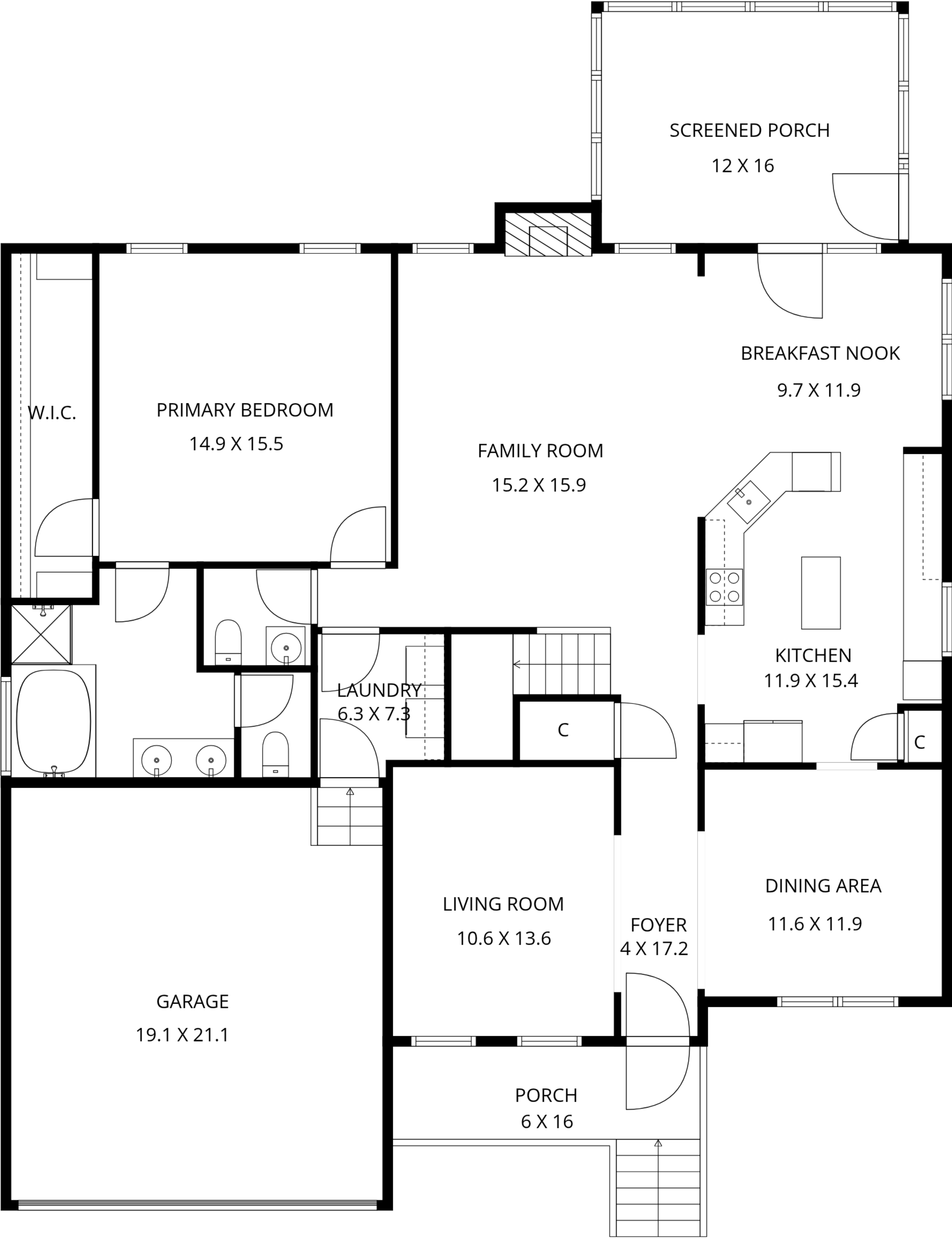
1ST FLOOR
