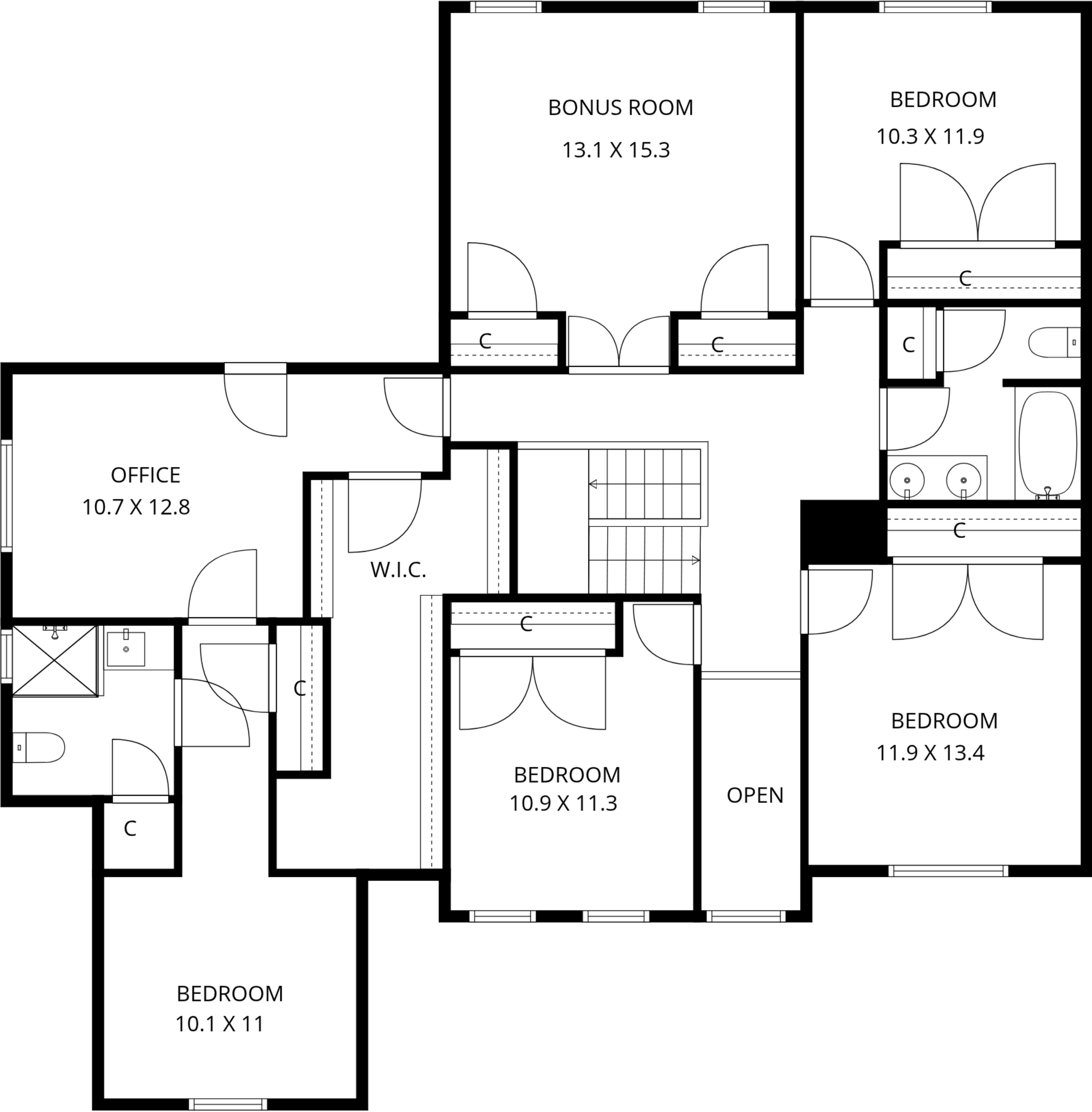
2ND FLOOR
