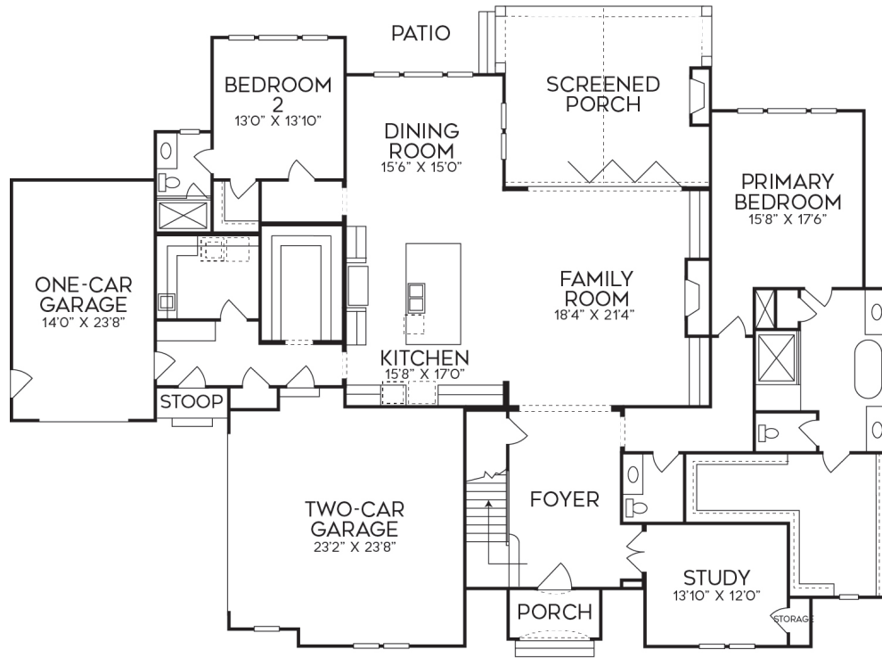
FIRST FLOOR
