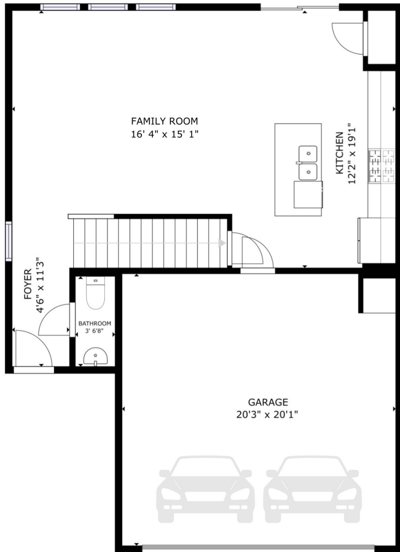
FLOOR 1 608 SQ.FT.
