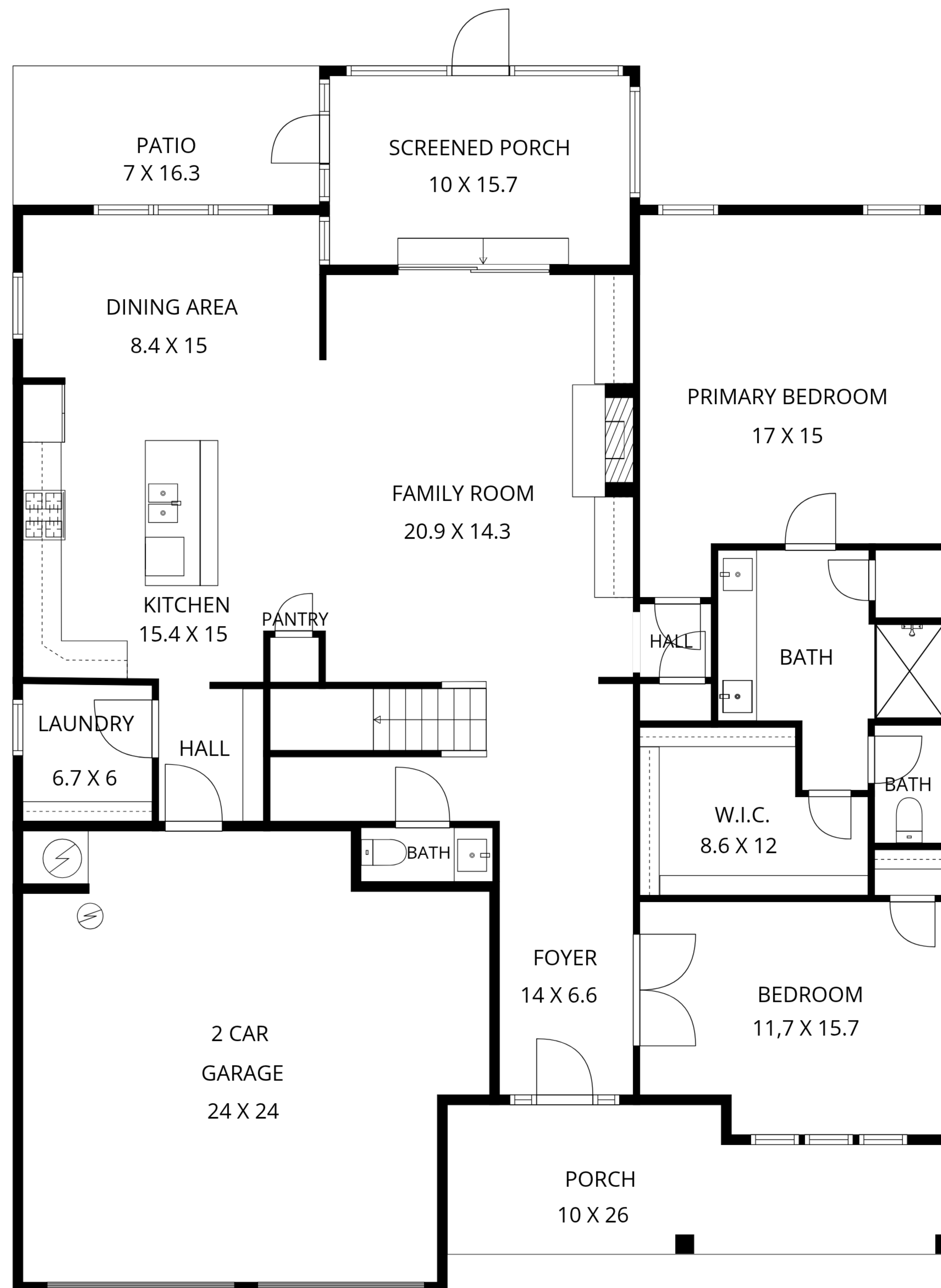
1ST FLOOR
