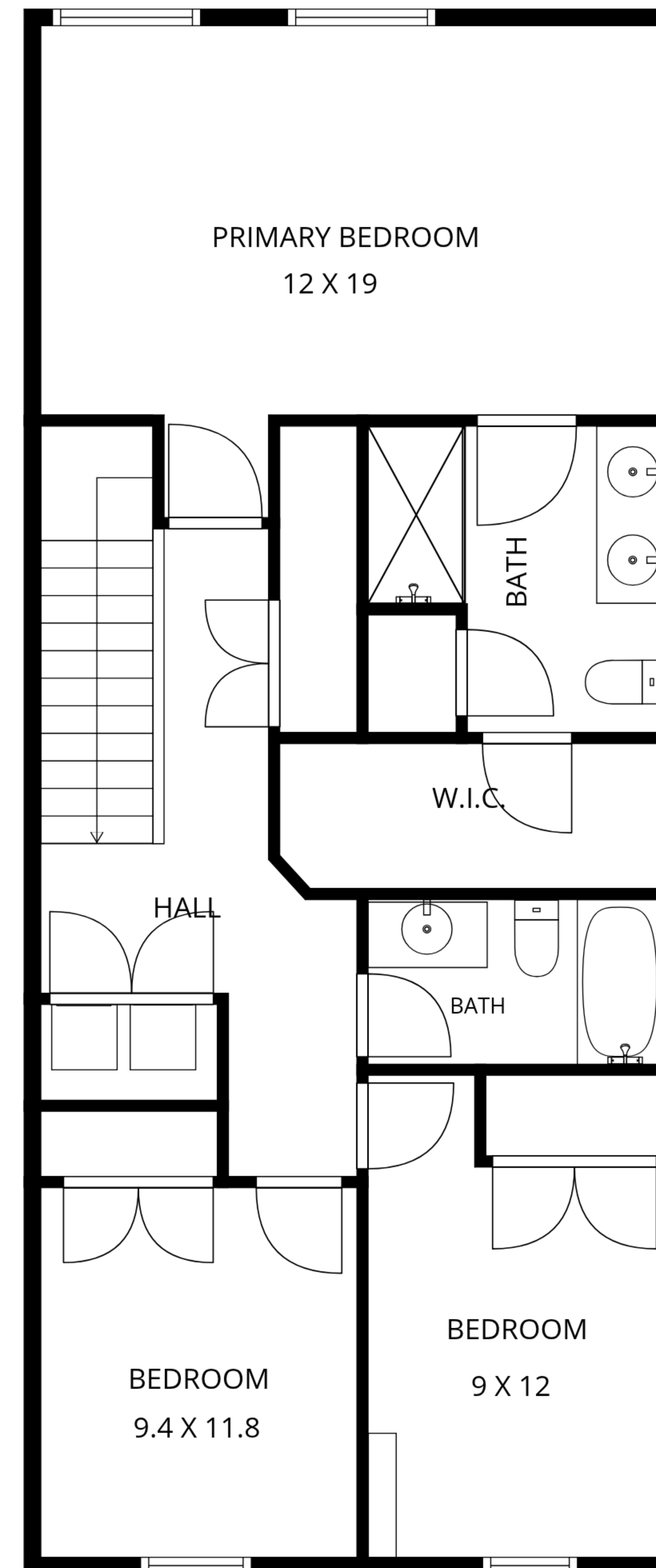
2ND FLOOR
