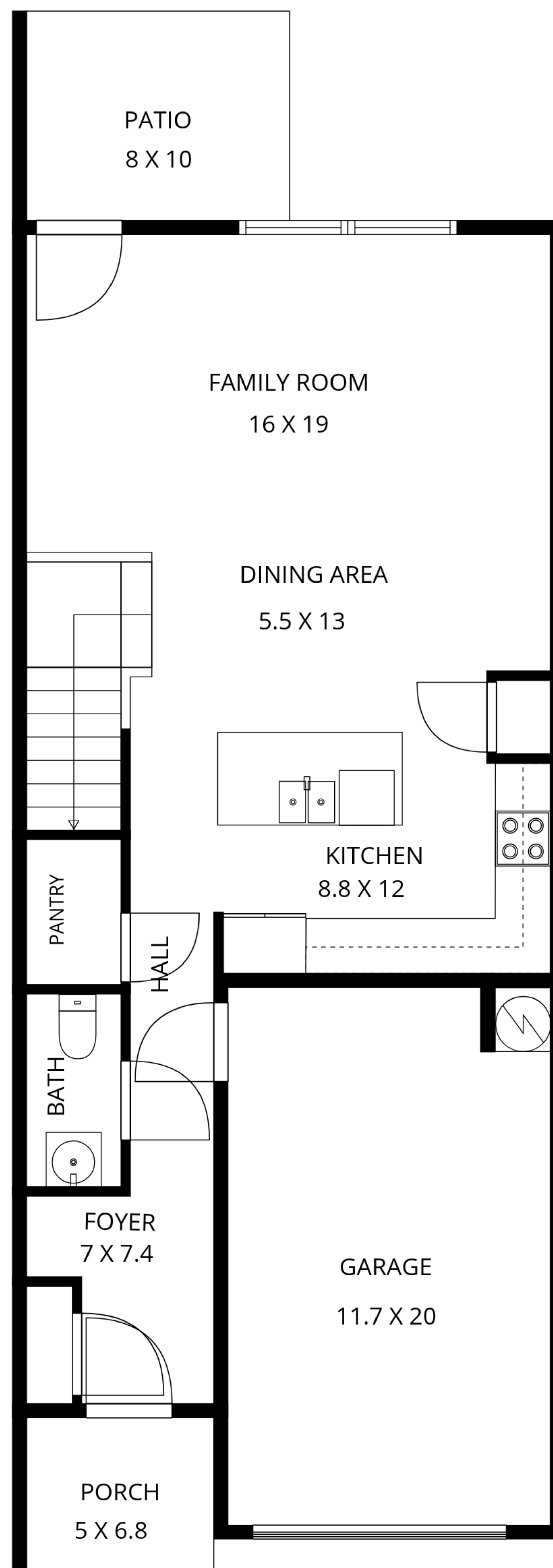
1ST FLOOR
