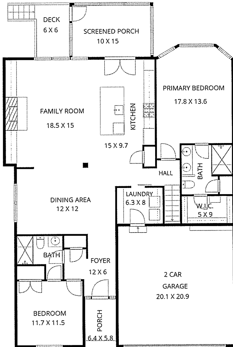
1ST FLOOR
