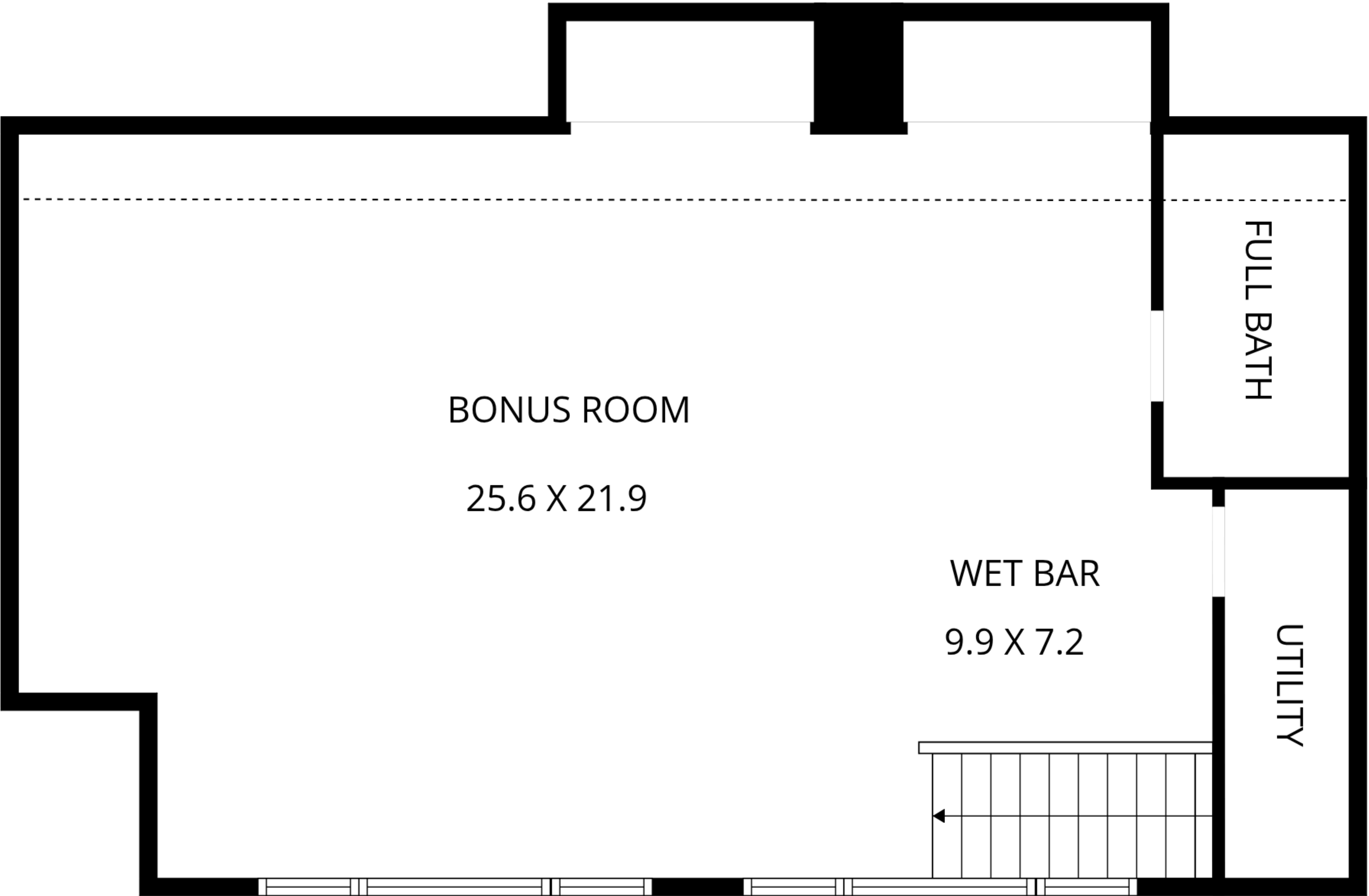
2nd floor
