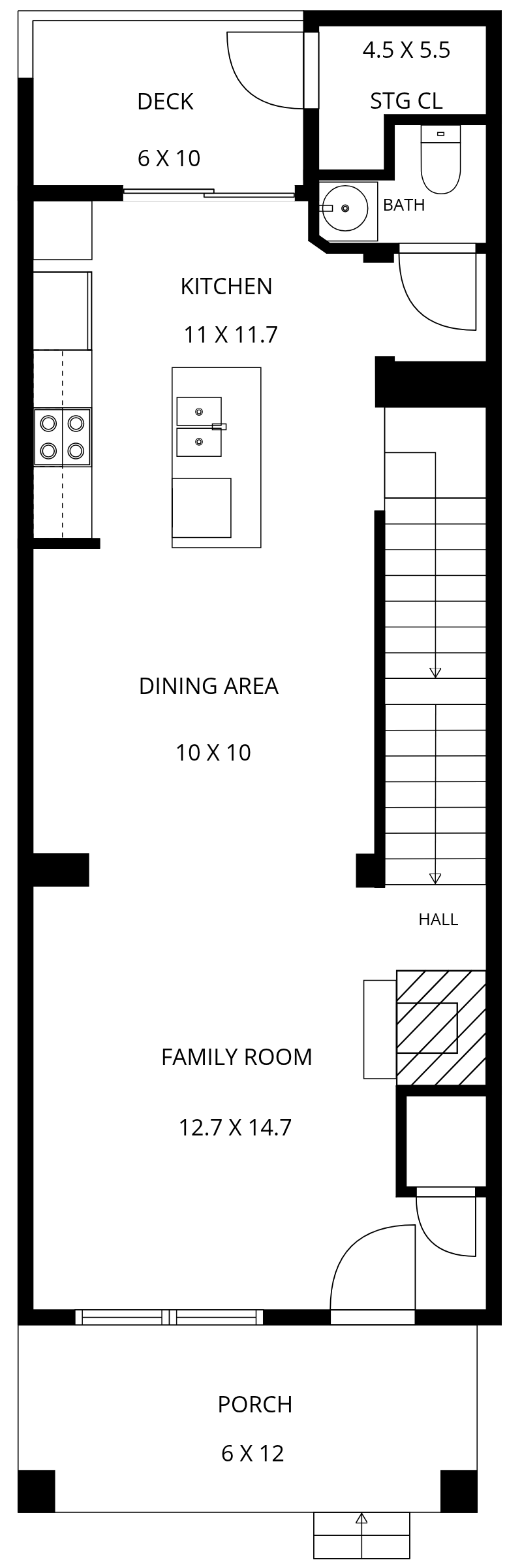
1ST FLOOR
