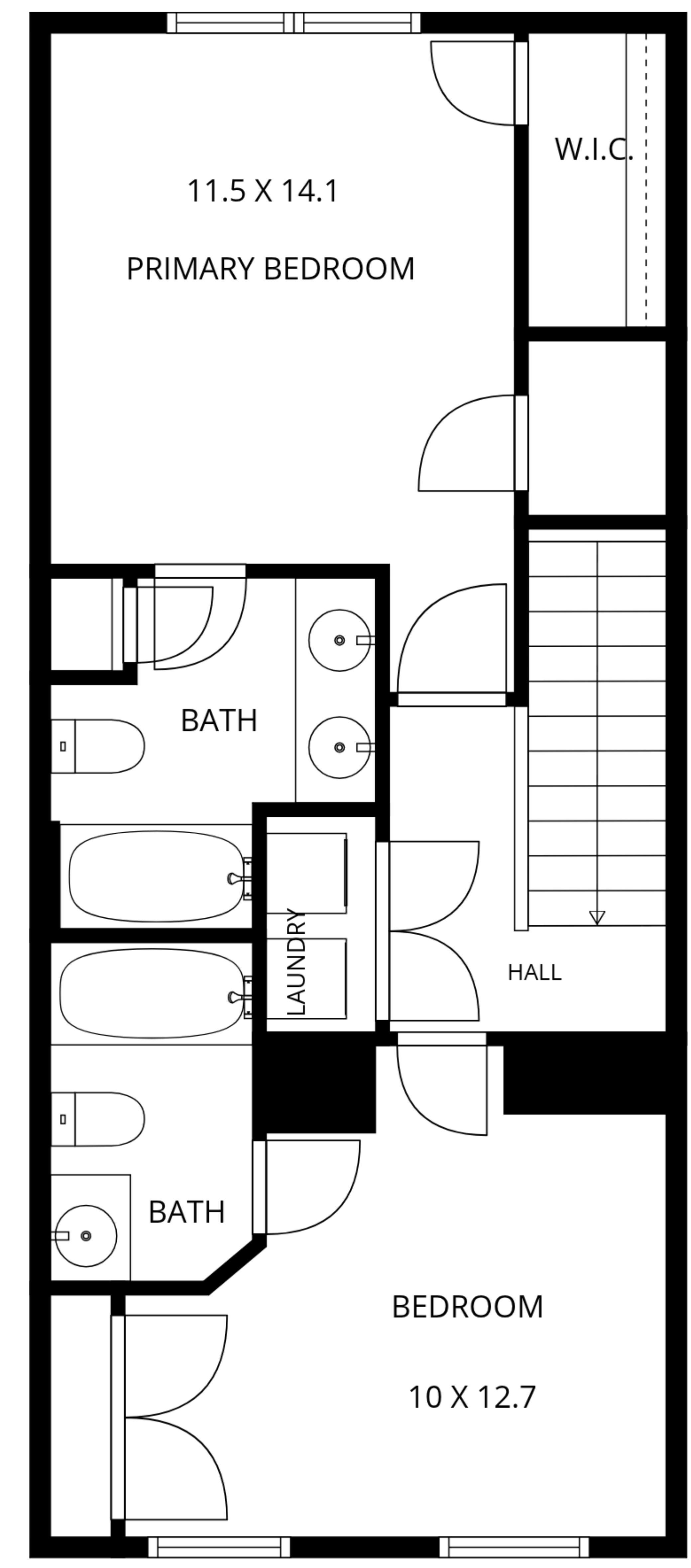
2ND FLOOR
