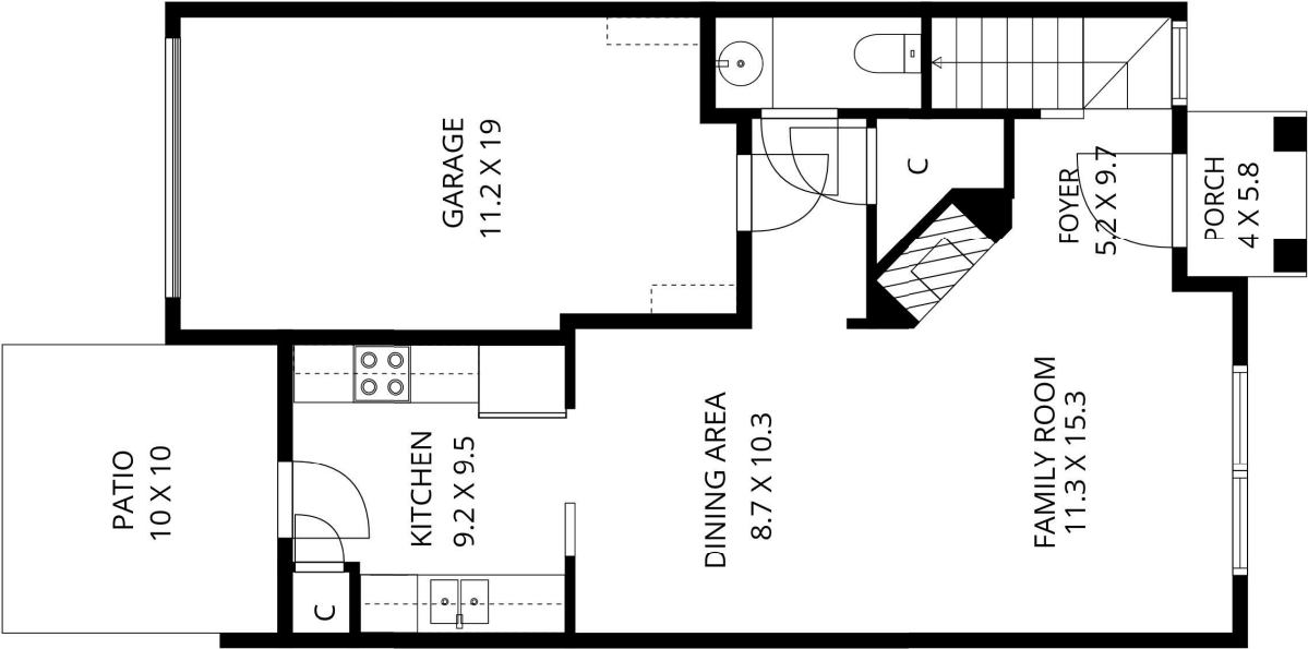
1ST FLOOR
