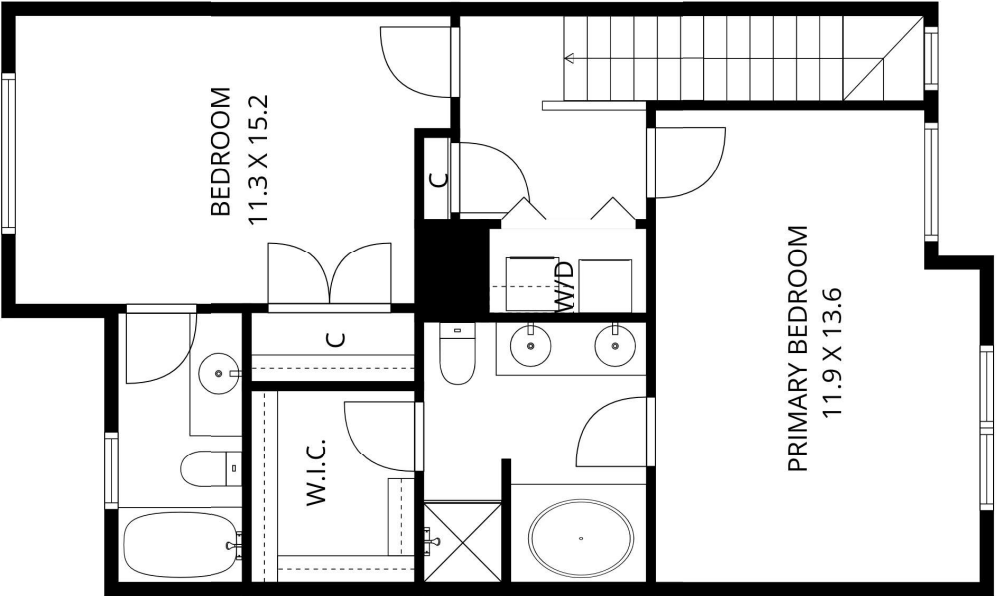
2ND FLOOR
