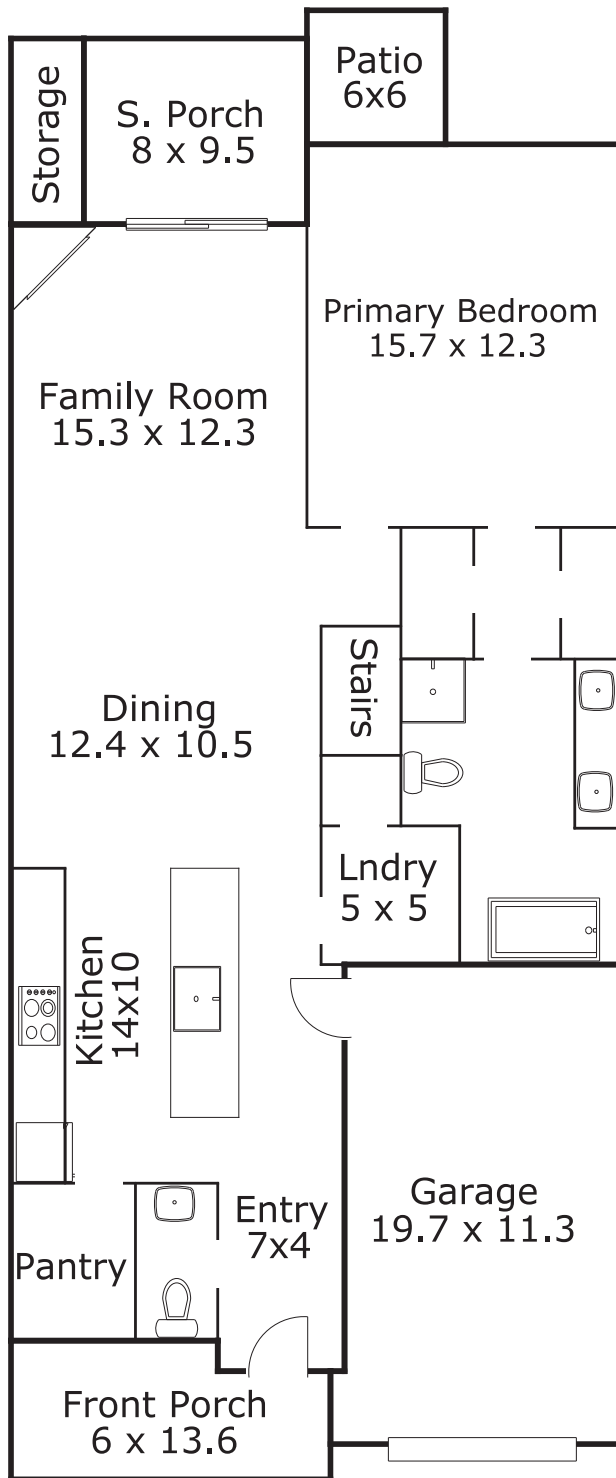
First Floor
