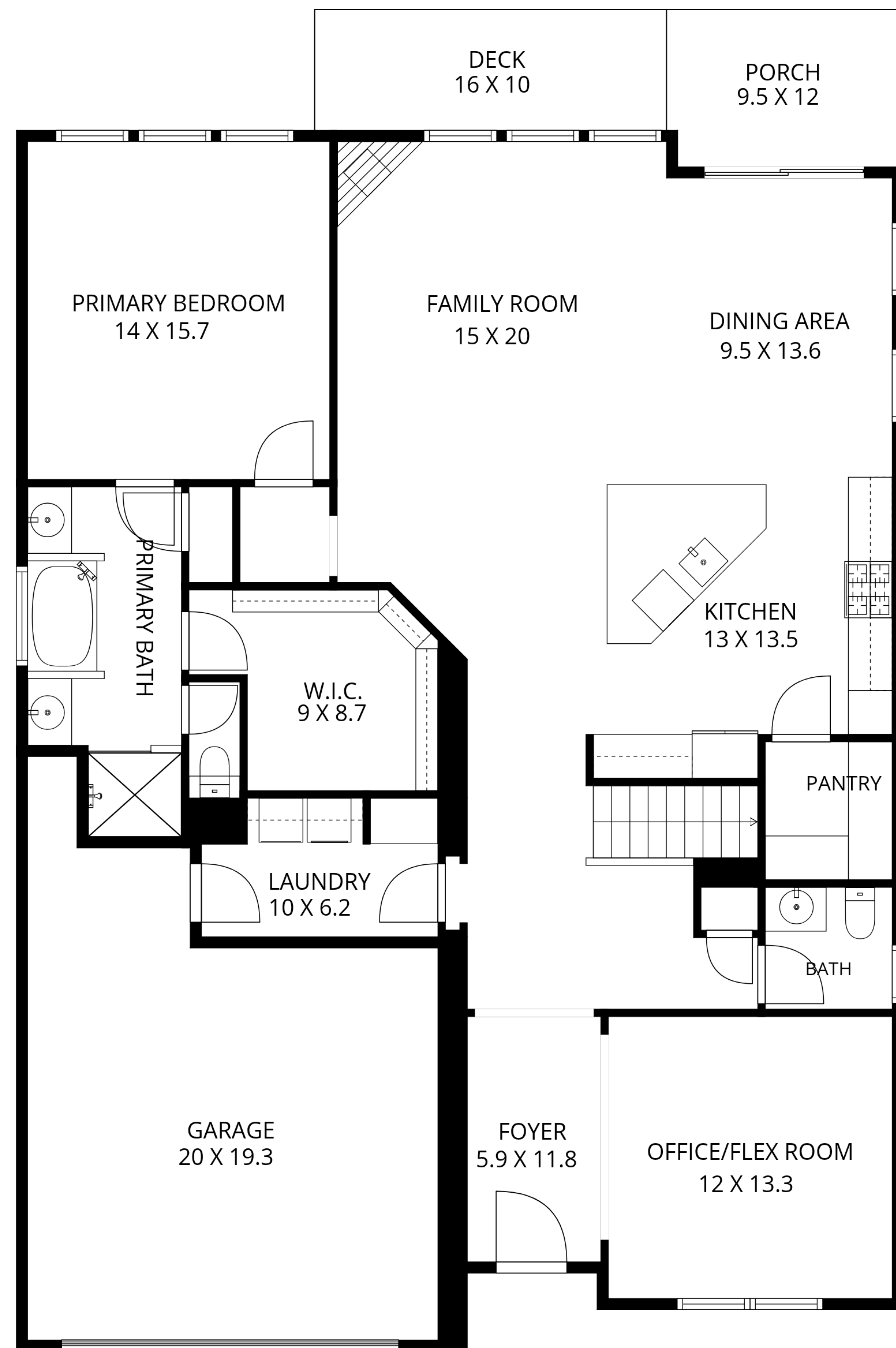
1ST FLOOR
