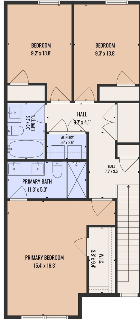
2ND FLOOR
