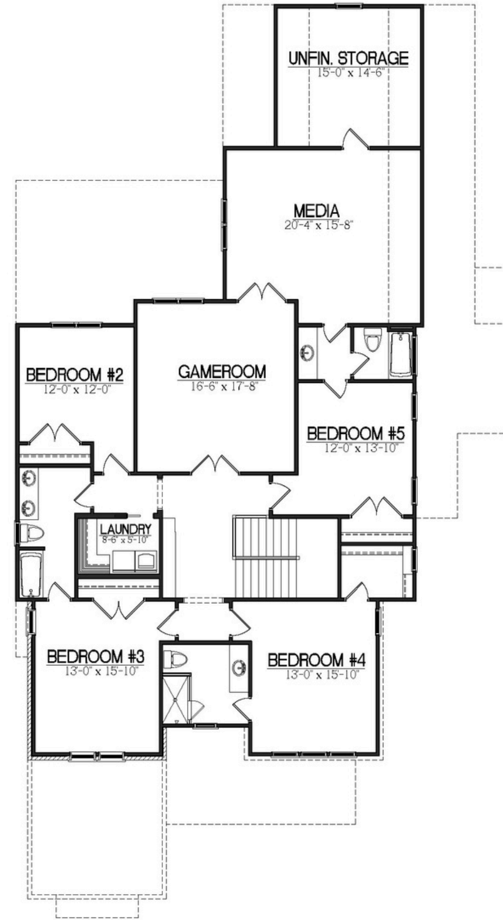
FLOOR TWO
